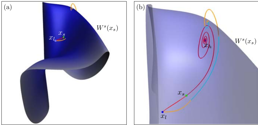
Fig. 6 Three-dimensional phase portrait of the fast subsystem with Ca = 0.55 \mu\text{M} . The V axis is horizontal. The blue surface in panel (a), which is rendered transparent in panel (b), is the stable manifold W^s(x_s) of the saddle steady state x_s (see also Fig. 3(b)) and defines the basin boundary of the high-voltage steady state x_h . Red curves are the unstable manifolds of x_s (green dot). Shown in orange is the trajectory for I_{\text{app}} = 12.87 \text{ pA} , with segments that lie inside the basin of attraction shown in cyan. A large enough applied current I_{\text{app}} will move the system out of the low-voltage steady state x_l , so that only very specific durations capture the trajectory inside the basin of attraction of x_h . (Color figure online.)
