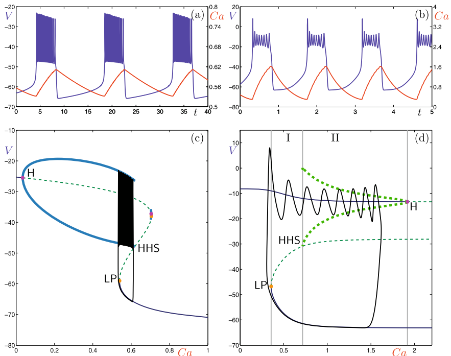
Fig. 2 The bursting profile for the Chay–Keizer model (left column) compared with that for the pituitary model (right column). Panels (a) and (b) show V (purple, left axis) and \text{Ca} (orange, right axis) versus t . Panels (c) and (d) show these orbits in the (\text{Ca}, V) -plane overlaid on the bifurcation diagrams of the corresponding fast subsystems. (Color figure online.)
