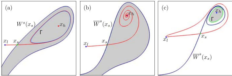
Fig. 3 Basins of attraction (shaded) of the depolarized state x_h in the fast subsystem. Panel (a) shows the Chay–Keizer model with Ca = 0.55 . Panel (b) shows a projection of a similarly large basin for the pituitary model with Ca = 0.55 (region I in Fig. 2(d)), but the basin is dramatically smaller for the pituitary model at Ca = 1.0 (region II in Fig. 2(d)) shown in panel (c). In each panel the horizontal axis is V and the vertical axis is n . The periodic orbit and the high-voltage and low-voltage and saddle steady states are labeled \Gamma , x_h , x_l , and x_s , respectively. Panel (a) shows the one-dimensional stable and unstable manifolds W^s(x_s) and W^u(x_s) of x_s , respectively, while panels (b) and (c) show projections of the one-dimensional unstable manifold W^u(x_s) and a one-dimensional slice \overline{W}^s(x_s) of the two-dimensional stable manifold of x_s .
