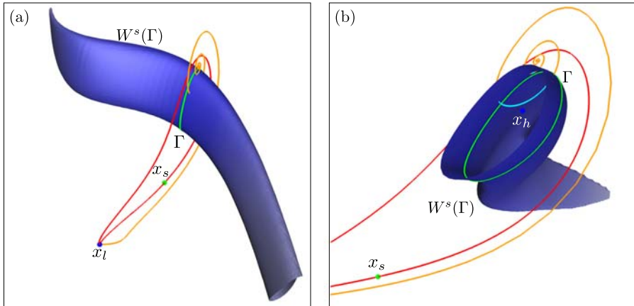
Fig. 8 Three-dimensional phase portrait of the fast subsystem with Ca = 1.0 \mu\text{M} . Colors are as in Fig. 6 but now the basin boundary (blue surface) is the stable manifold W^s(\Gamma) of the unstable periodic orbit \Gamma (dark green curve). The horizontal axis is V in panel (a), while the view is rotated in panel (b) and part of the basin boundary chopped off so one can see inside. Any applied current I_{\text{app}} large enough to move the system out of the low-voltage steady state x_l will converge to a point outside the basin of attraction of the high-voltage steady state x_h . Shown in orange is the trajectory for I_{\text{app}} = 6.69 with segments that lie inside the basin of attraction shown in cyan. Red indicates the unstable manifolds W^u(x_s) of x_s (green dot). (Color figure online.)
