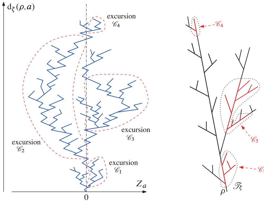
Fig. 6. A schematic representation of excursions. The right side shows the tree \mathcal{T}_\xi , and the parts of the tree inside the dotted lines are a few connected components of the set \{a \in \mathcal{T}_\xi : Z_a \neq 0\} . The left side shows the values of Z_a for a \in \mathcal{T}_\xi , or equivalently the paths W_s which form a “tree of Brownian paths”, and the parts inside the dashed lines are a few excursions away from 0
