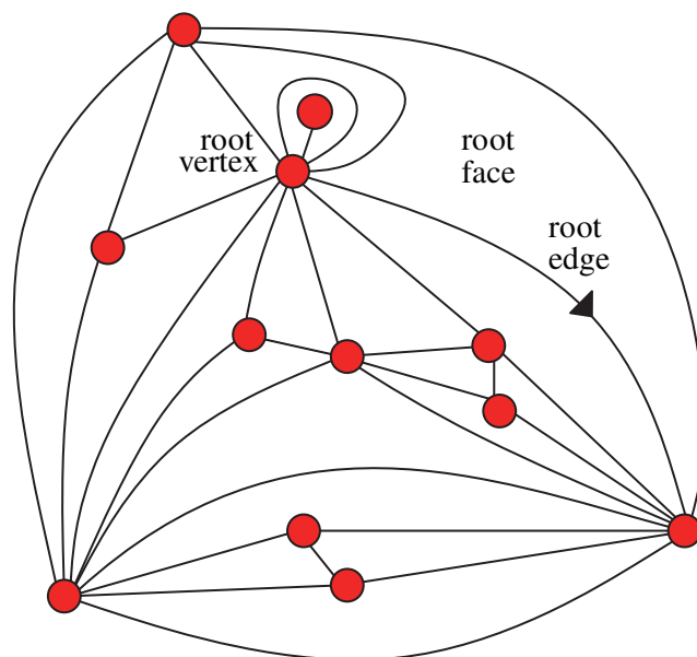
Fig. 1. A rooted triangulation with 20 faces
