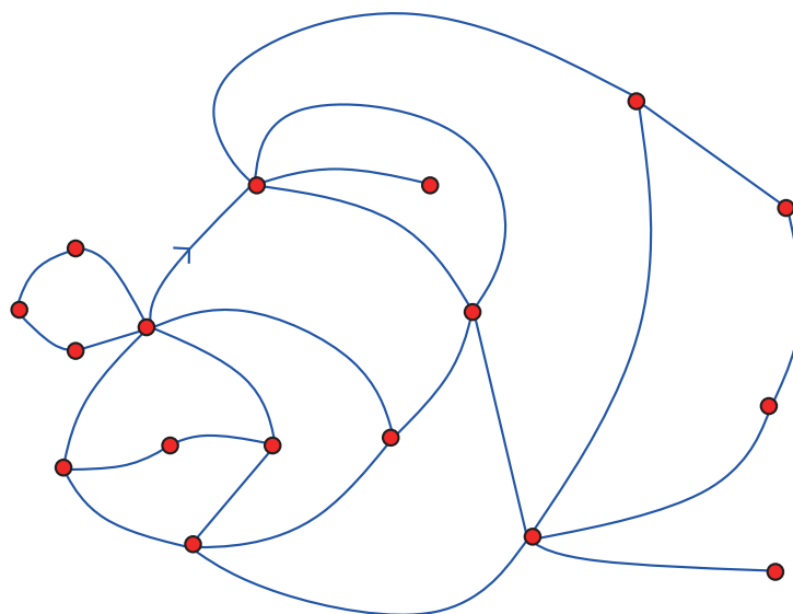
Fig. 5. A quadrangulation with a boundary of size 14
