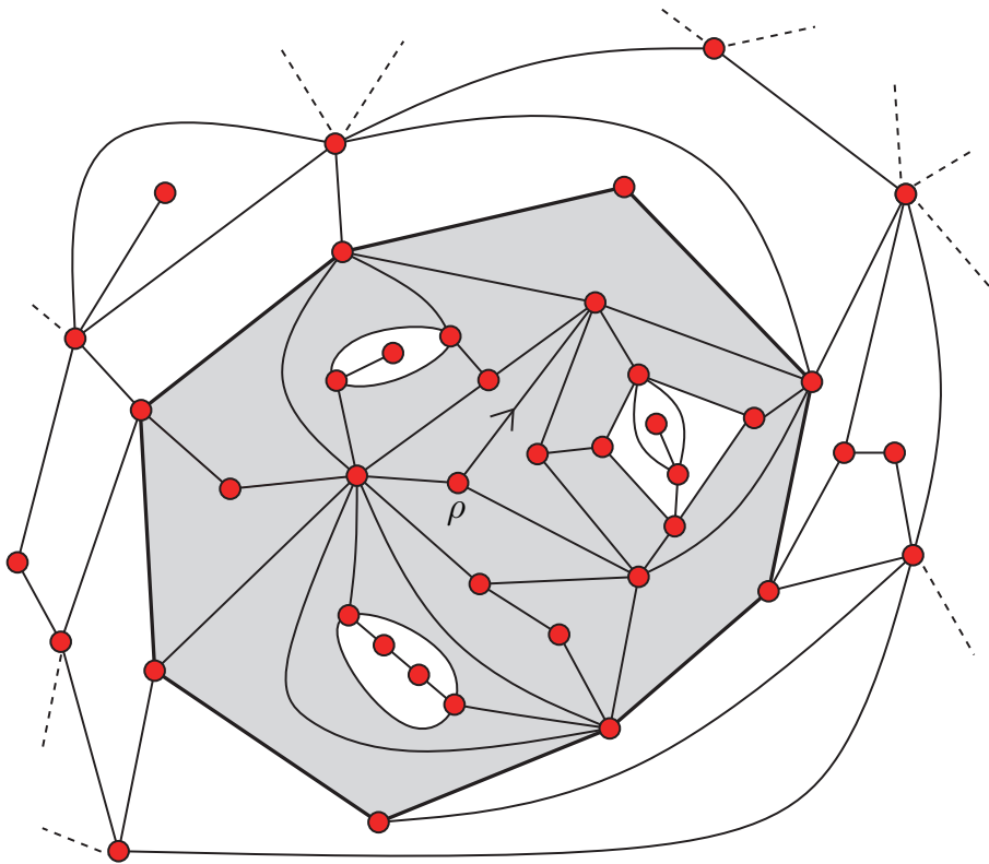
Fig. 3. A large quadrangulation Q near its root vertex \rho and in grey the ball B_2(Q)
