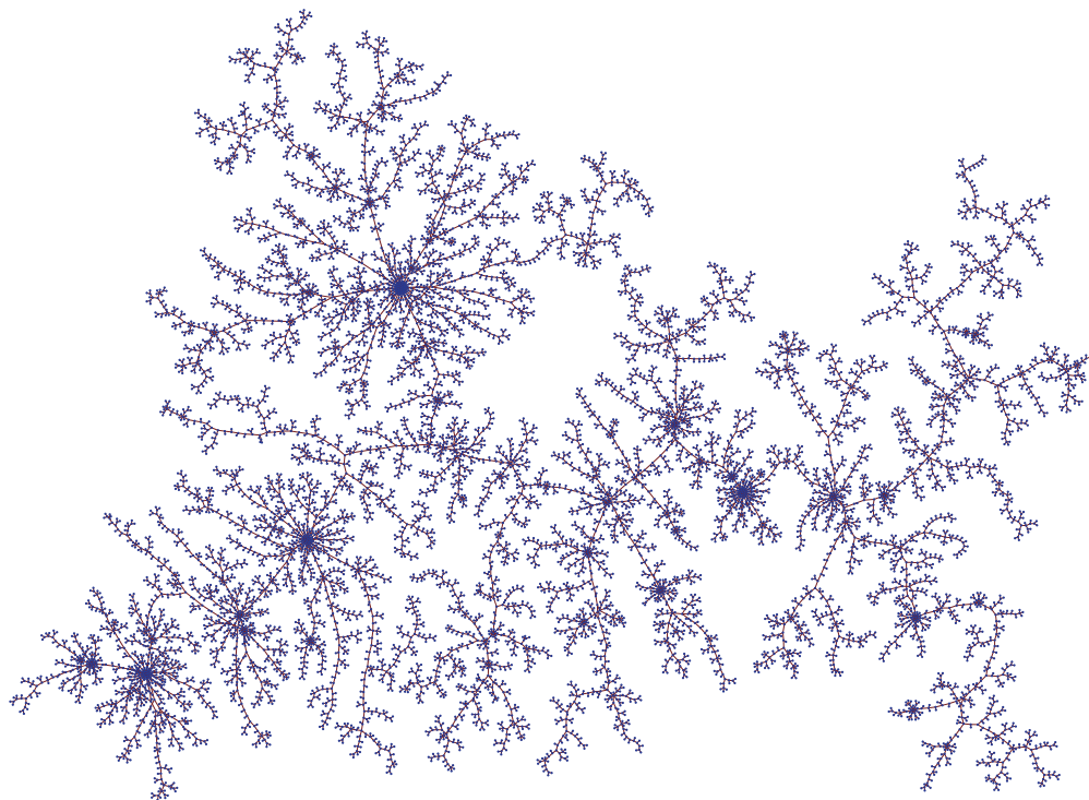
Fig. 8. A simulation of the stable tree with index 3/2 (simulation: I. Kortchemski)
