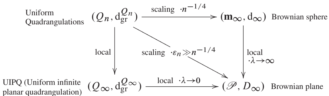
Fig. 4. Convergence to the Brownian plane
