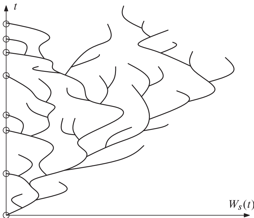
Fig. 7. A schematic representation of the paths W_s under \mathbb{N}_0^* . The quantity \mathcal{L}_0^* measures the “number” of circled points corresponding to returns of certain paths W_s to 0
