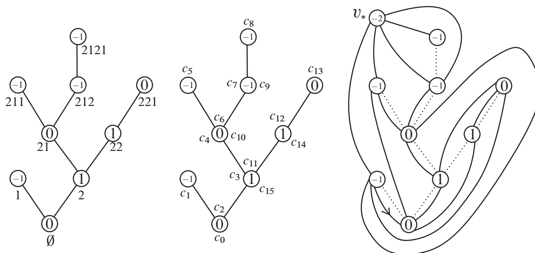
Fig. 2. Schaeffer's bijection. Left: a labeled tree with 8 edges. Middle: the sequence c_0, c_1, \dots, c_{15} of corners enumerated in cyclic order. Right: the edges of the associated quadrangulations with 8 faces (case \varepsilon = -1 )
