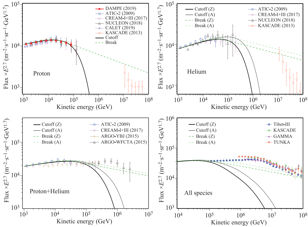
Fig. 1 Energy spectra of protons (top-left), Helium (top-right), proton plus Helium (bottom-left), and all species (bottom-right). In each panel the solid lines show the fitting results with an exponential cutoff form [Eq. (1)], and the dashed lines show the broken power-law [Eq. (2)] fitting results. The thick lines are for the Z -dependent cutoff/break energies, and the thin lines are for the A -dependent cases. References of the data: protons, ATIC [2], CREAM [31], NUCLEON [32], CALET [8], DAMPE [35], KASCADE [43]; Helium, ATIC [2], CREAM [31], NUCLEON [32], KASCADE [43]; p+He, ATIC [2], CREAM [31], ARGO-YBJ [44], ARGO-WFCTA [41]; all-particle, Tibet-III [38], KASCADE [36], GAMMA [39], TUNKA [37].
