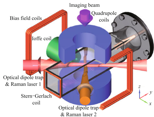
Fig. 1 Schematic drawing of the experimental setup for SO coupled BEC. Two horizontal crossed beams at 90^\circ are used as the optical dipole trap and the Raman beams.
