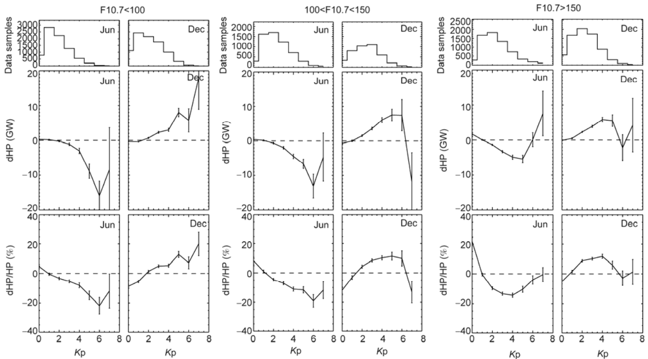
Figure 3 Hemisphere difference of HP (North minus South) under different K_p levels from 1979–2007. The three groups of plots are refer to different solar activities ( F10.7 < 100 , 100 < F10.7 < 150 , F10.7 > 150 ). For each group of the plots, the upper two panels show the number of data samples for different K_p . The middle panels show the difference of HP (north minus south) under different K_p levels around summer solstice (Jun) and winter solstice (Dec). The bottom presents percentage difference of HP for summer and winter, respectively.
