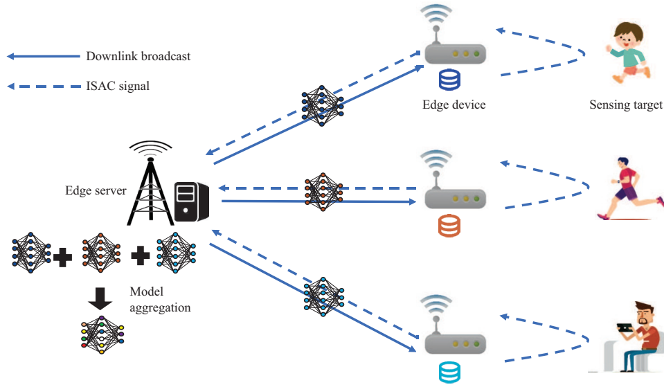
Figure 7 (Color online) Illustration of the FEEL system with ISAC.
