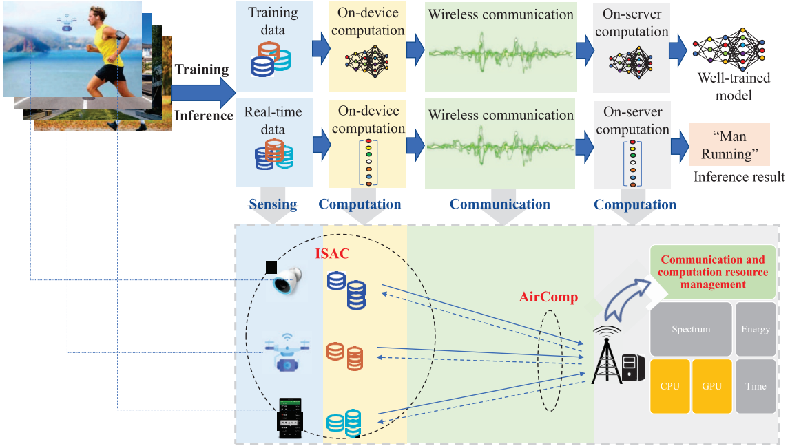
Figure 3 (Color online) Sensing, communication, and computation in edge AI.
