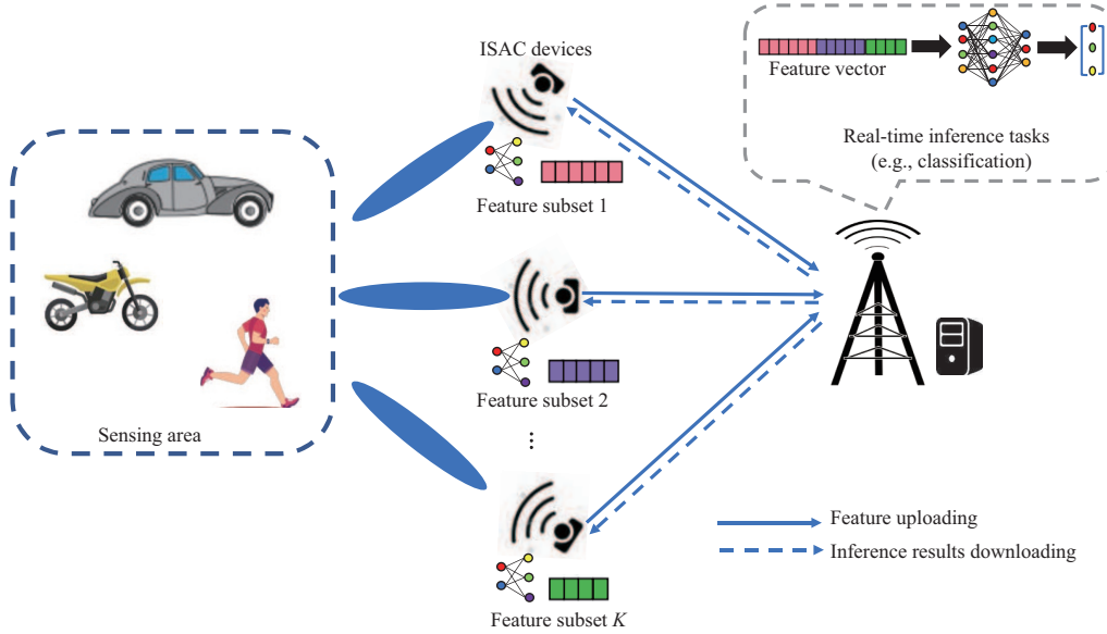
Figure 9 (Color online) Edge inference systems with multi-device sensing.
