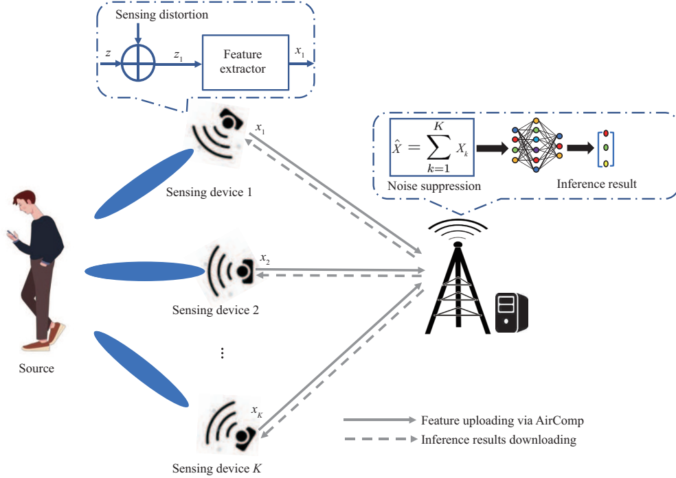
Figure 8 (Color online) Illustration of AirComp-based edge inference systems.
