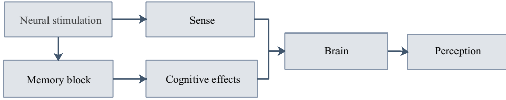
Figure 3 The generation process from sensation to perception. Perception is the cognitive result of the external things formed by the brain. It is the combination of two parts of information. The first part is the input information of the outside world, and the second part is the memory.
