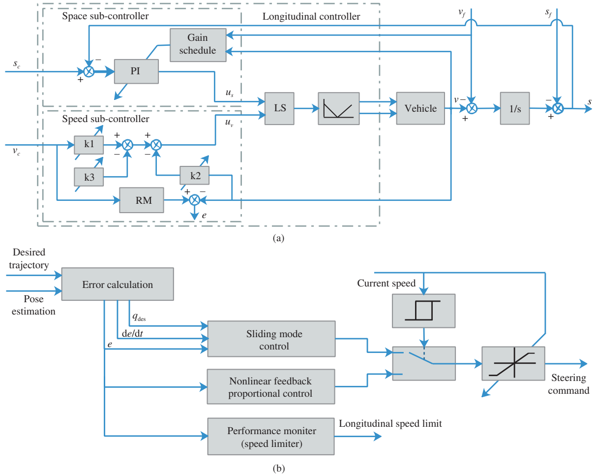
Figure 7 Longitudinal and lateral control computing framework. (a) describes the longitudinal control computing framework, which consists of speed sub-controller and space sub-controller. Speed controller takes speed as the input and transforms the command to the control of throttle and brake, whereas the space-sub controller acts as a basic distance insurance (autonomous emergency braking). (b) shows the details of the lateral control computing framework. It uses the sliding mode control and nonlinear feedback proportional control with an amplitude limited unit to obtain the steering command, and the performance monitor is operated as the constraint of the longitudinal speed.
