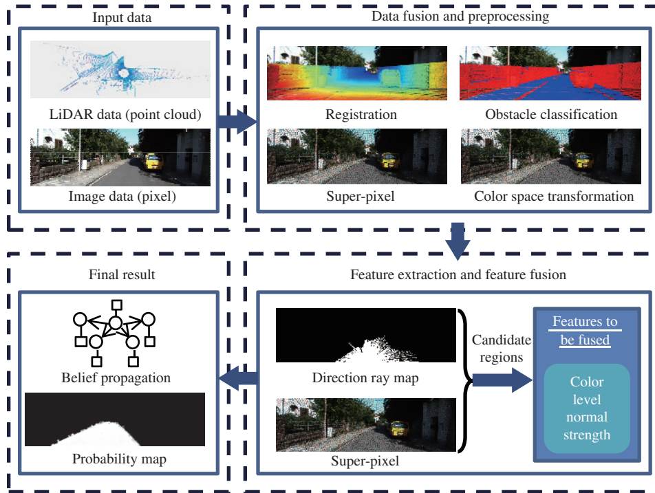
Figure 5 Unsupervised method for drivable area detection. The scene is analyzed in different feature spaces, and the different features obtained are merged. Finally belief propagation is used to analyze the fused features to obtain probability of the drivable area.
