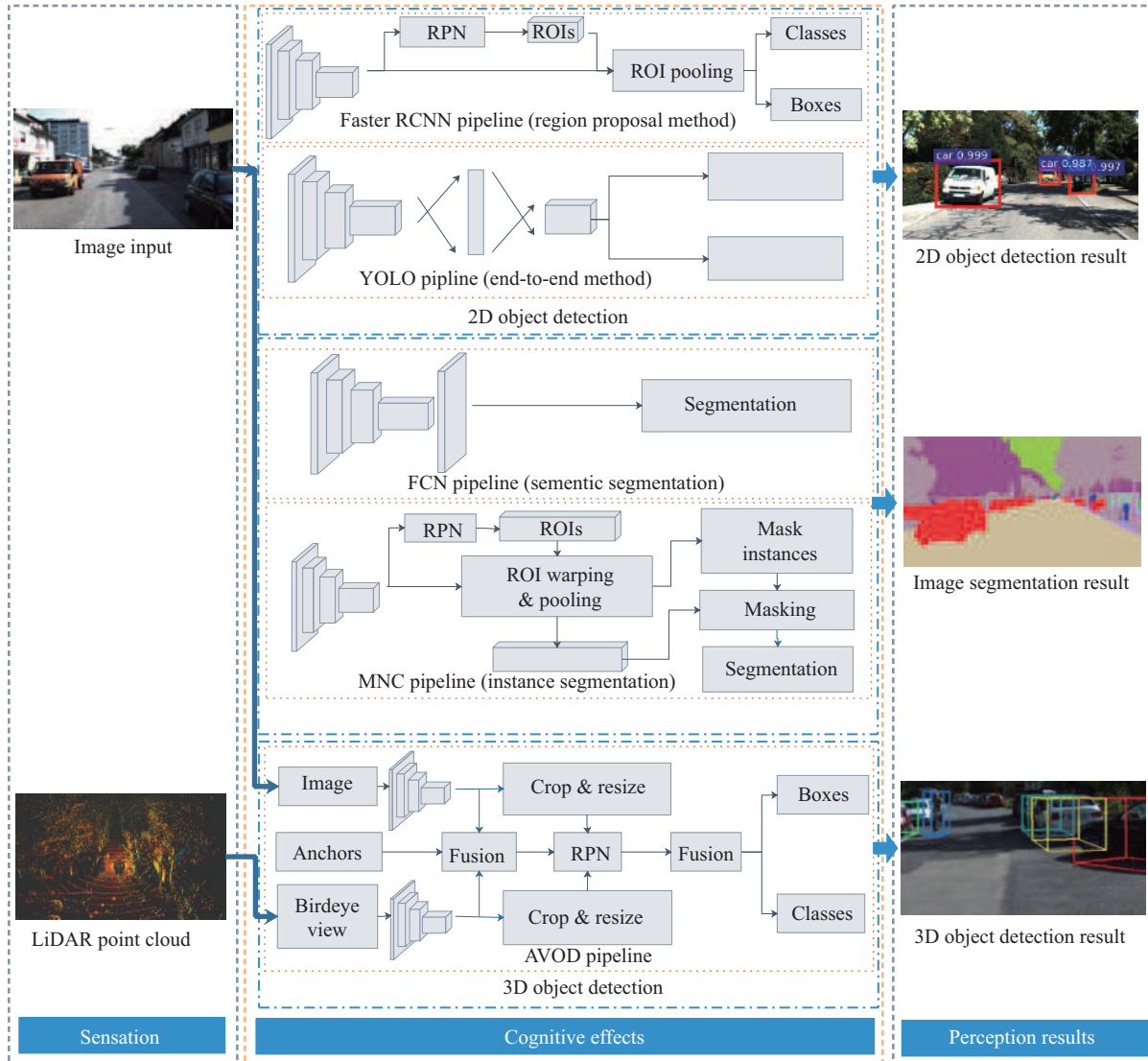
Figure 4 Objects detection and image segmentation in traffic scenarios. Three types of traffic scene perception algorithms are listed here, the input of which is mainly images and LiDAR point cloud. Different types of algorithms have different outputs for specific tasks, and these outputs will also play different roles in the perception of autonomous driving systems.
