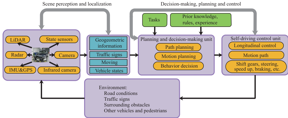
Figure 1 Data-driven computing framework of self-driving cars. The scene perception obtained by the sensors is used in localization, after planning and decision-making step, the control signal received by the self-driving control unit is utilized to control the self-driving cars. Meanwhile, environments like road conditions are feedback into the perception module for further processing.
