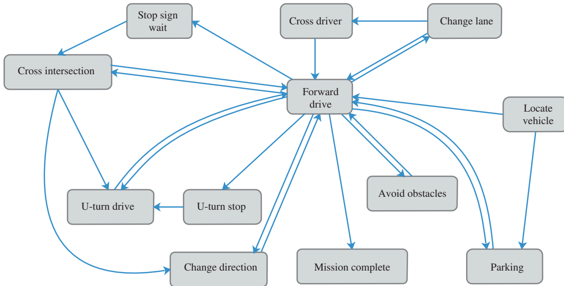
Figure 6 Illustration of decision-making finite state machine. The finite state machine is consist of several driving behavioral states. With the different input information, it defines the transition relationships of the current and the next behavioral state.
