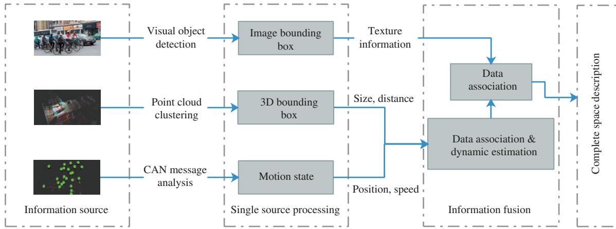
Figure 12 Decision-level multi-source fusion-based object detection framework. It is made up of single source processing and information fusion stages, where each single-source sensors obtain the object separately at the single source processing step and followed by the fusing process which finally obtains the complete description of the scene.
