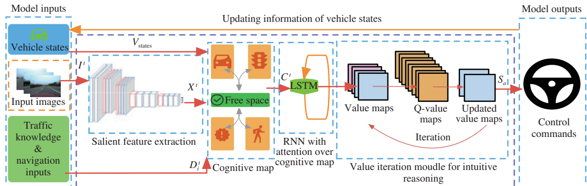
Figure 13 Cognitive computing framework of self-driving cars with selective attention mechanism and intuitive reasoning. The cognitive process is divided into four parts. The first part is the feature extraction by convolutional neural network, and the second part is the combination of features and prior knowledge to form a cognitive map. The third part is to filter the cognitive map by implementing the attention mechanism through LSTM. The last part is to reflect the cognitive map to the behavior space through the value iteration model, and output the final behavior decision.
