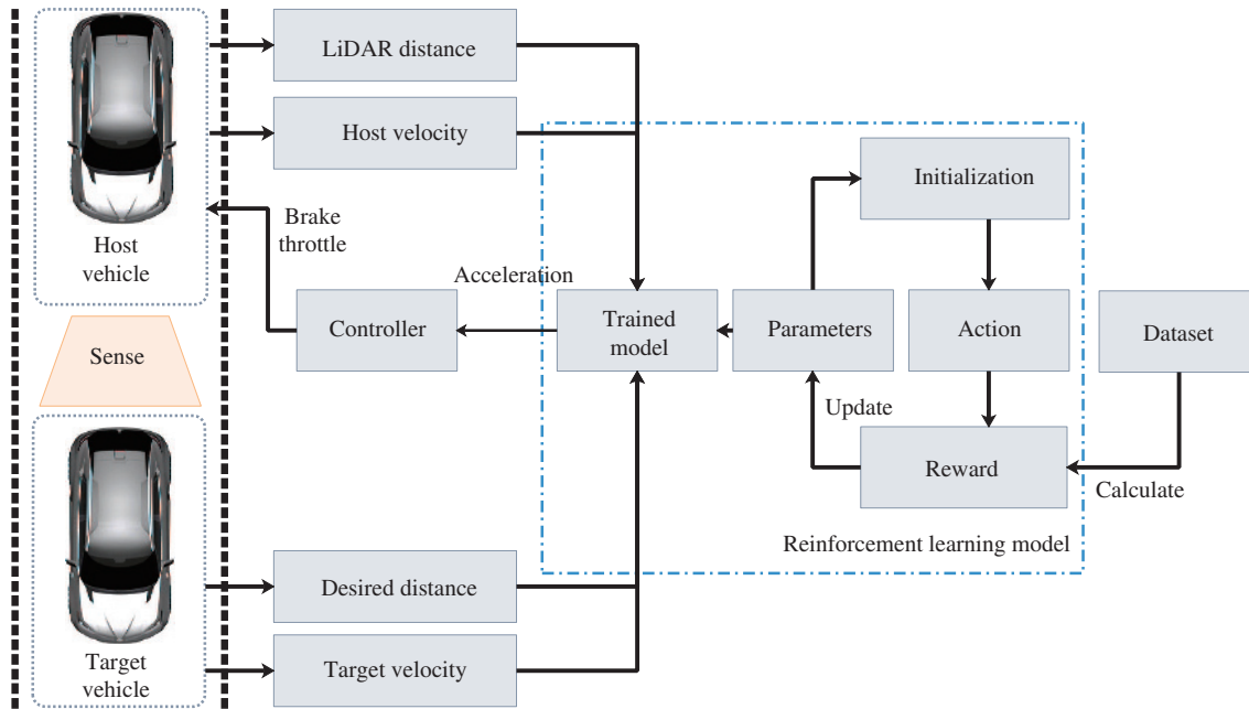
Figure 14 Reinforcement learning framework for adaptive cruise control. The desired speed and distance and the current speed and distance are input into the trained reinforcement learning model, and the acceleration is output to the control module to achieve vehicle following.
