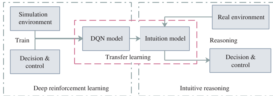
Figure 15 The generation of autonomous vehicle's intuition based on "reinforcement-transfer" learning. The autonomous driving model is trained in the simulation environment using the deep reinforcement learning, and then the model is transplanted to autonomous vehicles through migration learning.
