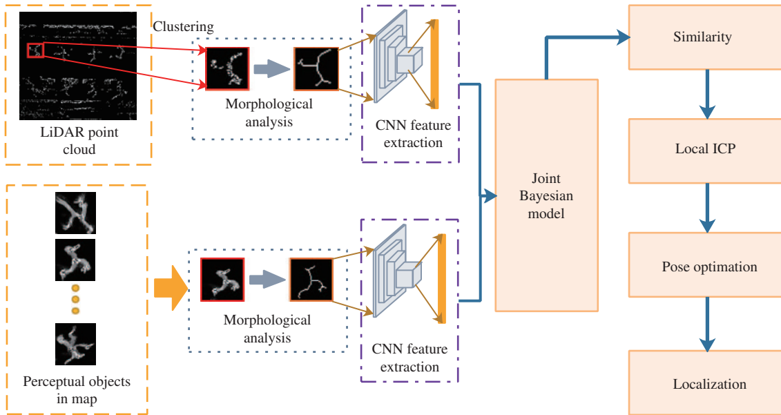
Figure 10 Localization method with perceptual objects. Through the similarity analysis of the perceptual objects in the map and the scene, we can get the correspondence between the map and the point cloud in the scene, so as to obtain the localization information by using the point cloud registration method.
