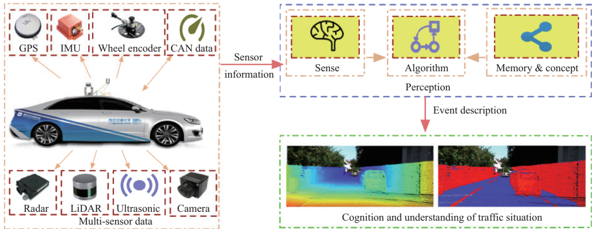
Figure 2 Cognition and understanding of traffic situation based on the information from the results of multi-sensor fusion. Using a variety of sensors to obtain data of different feature spaces and using different algorithms for analysis, and finally get cognitive results for the situation.
