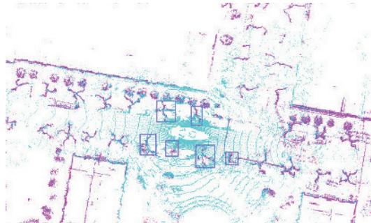
Figure 11 Visualization of the localization results using perceptual objects. The purple point cloud is the map, and the blue point cloud is the scene currently perceived by the vehicle. It can be seen that the two have a high degree of coincidence, which proves the accuracy of the positioning.
