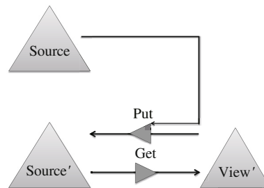
Figure 3 The PUTGET law.
