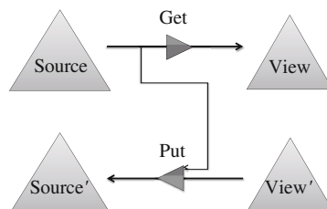
Figure 1 Forward and backward directions in BXs.
