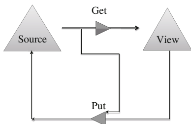
Figure 2 The GETPUT law.
