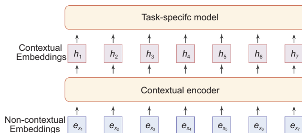
Figure 1 (Color online) Generic neural architecture for NLP.
