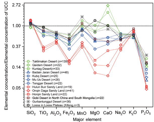
Figure 2 Elemental ratios of desert sediments in China and Mongolia.
