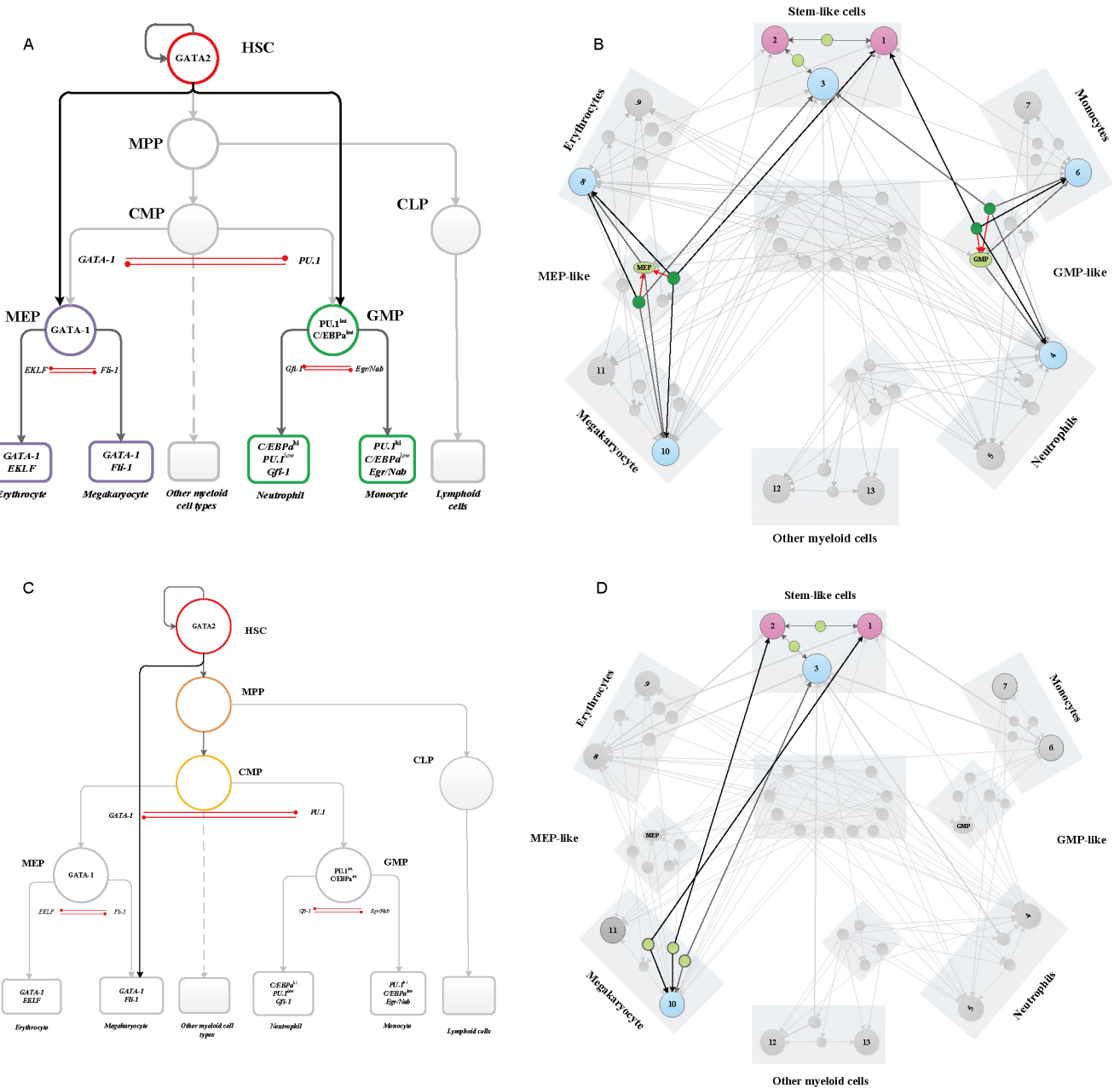
Figure 6 The endogenous network dynamics incorporated the seemingly conflicted roadmap models. The myeloid bypass model (A) in which HSCs directly give rise to myeloid-specific progenitors can be incorporated in the landscape model (B). The megakaryocyte-biased model (C) in which HSCs directly give rise to megakaryocyte-specific progenitors can be incorporated in the landscape model (D). We further predicted three independent routes to achieve megakaryocyte-biased development.
