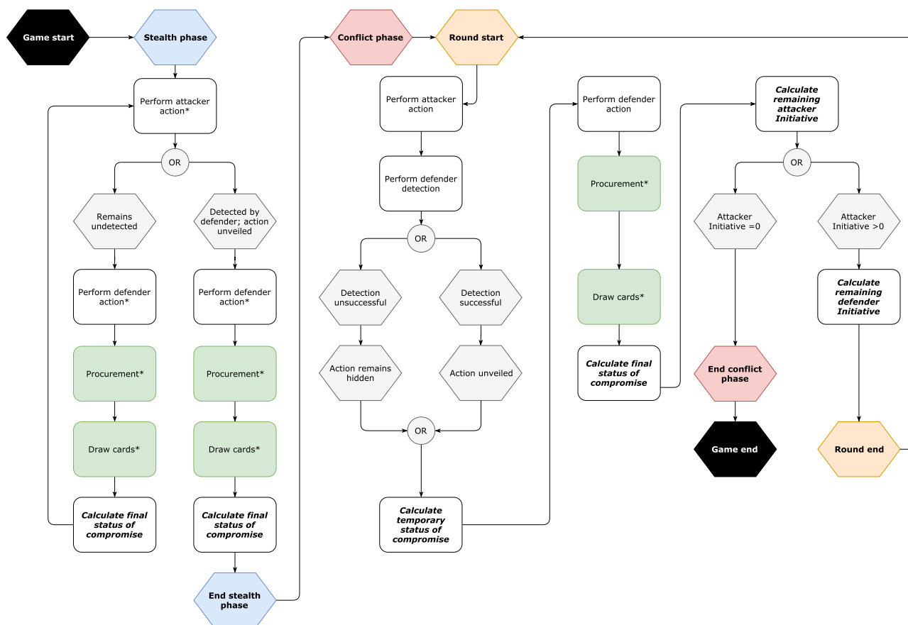
Fig. 6 Game phases and round progression overview. Actions marked with an asterisk (*) do not reduce the respective actor’s Initiative pool. Initiative and equipment status of compromise is recalculated after both actors have completed their actions
