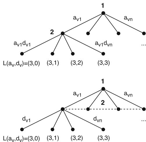
Fig. 3 Information set of the defending player for victim system compromise through attacker action a_{v1} , shown in extensive form [22]. In the above case, Player 2 successfully unveils a_{v1} , giving him the chance to specifically counteract the gain L(a_v) of Player 1 by increasing his own score L(d_v) through defense action d_{v1} . Below tree represents the limited information set for Player 2, when a_{v1} remains undetected
