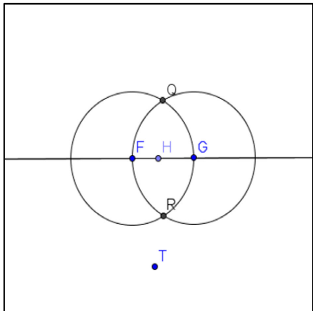
Fig. 9 Construction of two circles with the same radius (FG) centered at F and G
