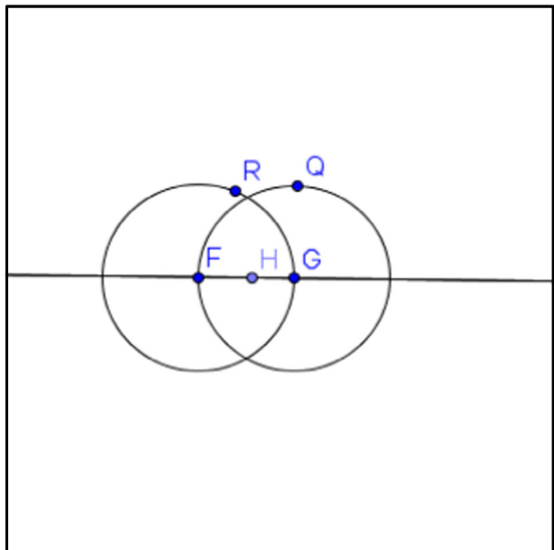
Fig. 7 Construction of two circles with different radii (GQ and FR) centered at F and G
