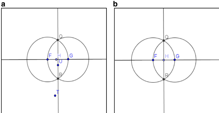
Fig. 10 a Construction of line QR. b Attaching point H to line QR
