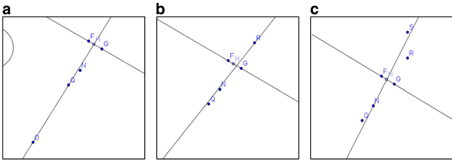
Fig. 4 a Construction of the perpendicular-looking line OQ. b Construction of a perpendicular-looking line passing point R. c Construction of the perpendicular-looking line HN
