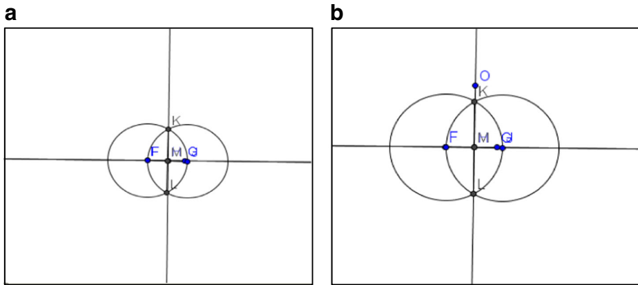
Fig. 6 a Placing PBC on top of H and aligning with line FG. b Constructing line OH using PBC as a guide
