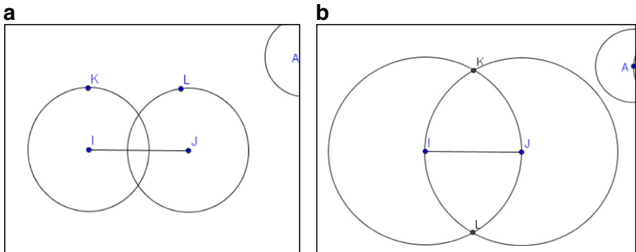
Fig. 2 a Two circles with different radii (IK and JL) centered at I and J. b Two circles with the same radius IJ centered at I and J
