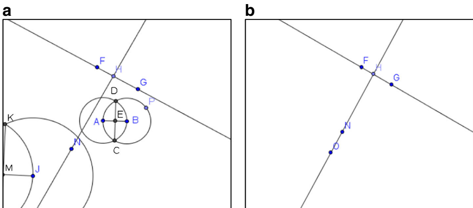
Fig. 3 a Construction of line NH that looks perpendicular to line FG. b Construction of another line (line OH) that looks perpendicular to line FG
