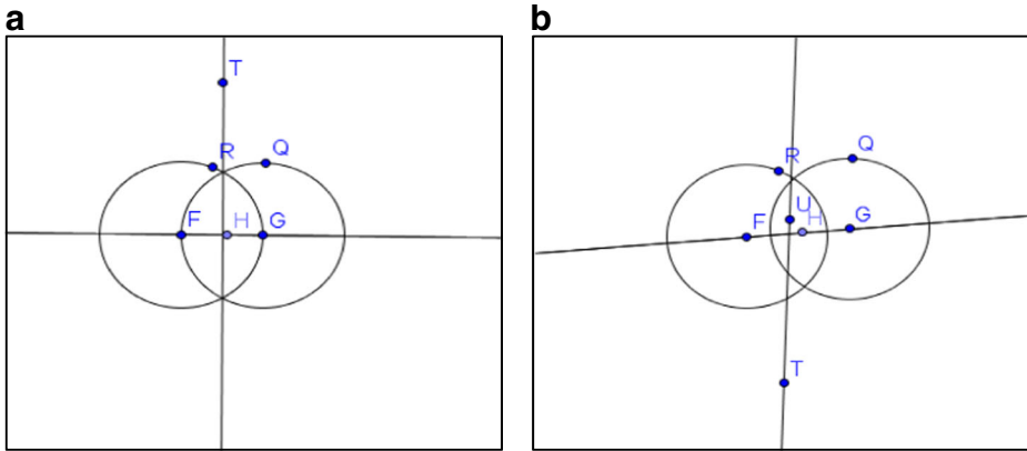
Fig. 8 a Construction of line TS. b Dragging line FG
