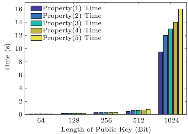
Fig.6. Paillier homomorphic properties time.
