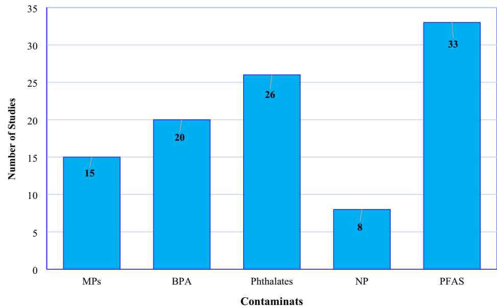
Fig. 2 The number of studies investigating migration of contaminants [microplastics (MPs), bisphenol A (BPA), phthalate, nonylphenol (NP), and perfluoroalkyl and polyfluoroalkyl substances (PFAS)] from pipes into drinking water distribution systems in the present study (More than one contaminant has been investigated in some studies)
