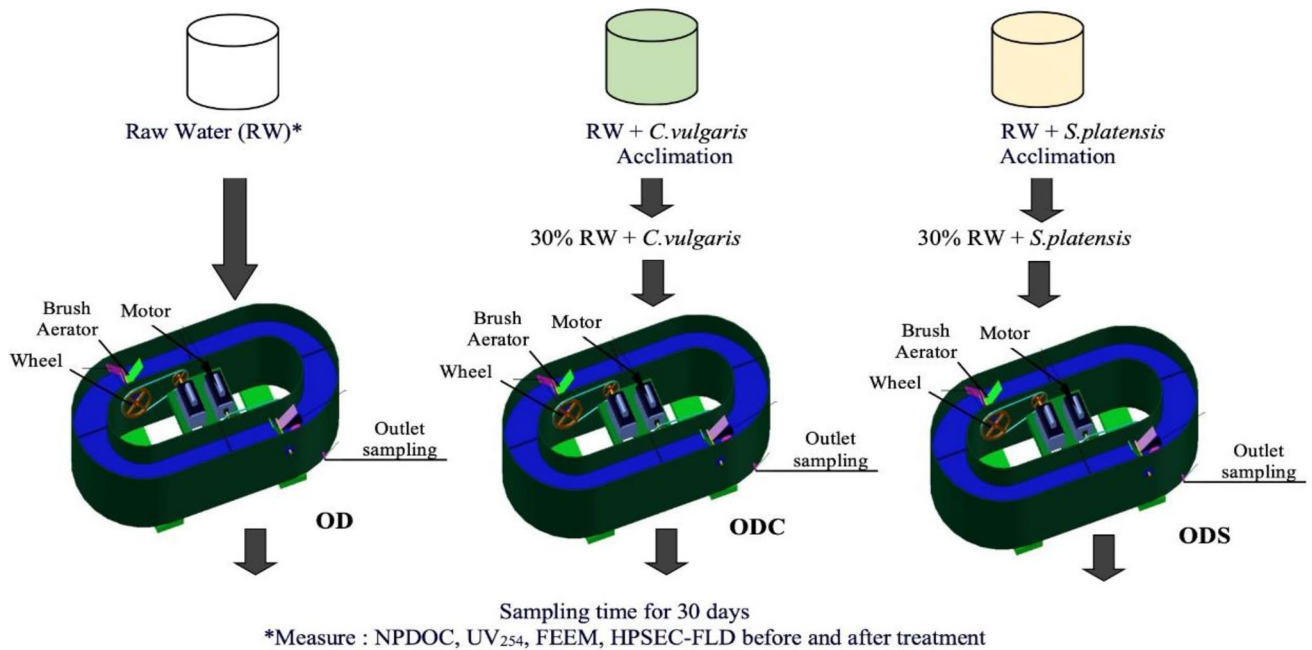
Fig. 1 The oxidation ditch system diagram
