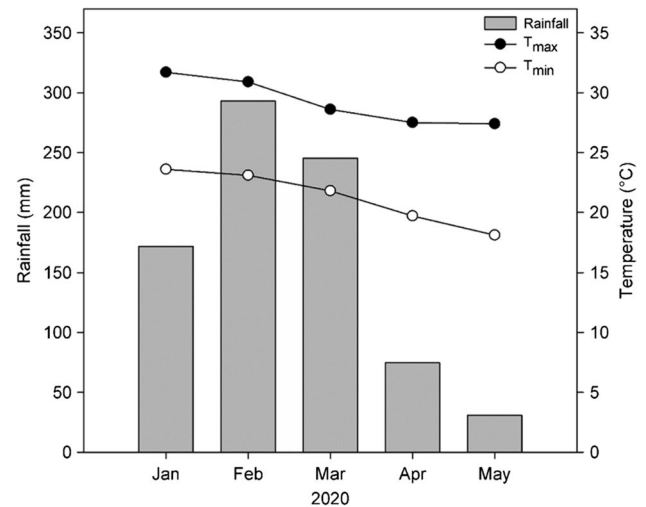
Fig. 1 Climate diagram of monthly average rainfall (bars), minimum and maximum temperature (dots) for Mariana, Minas Gerais, Brazil. Sources: Brazilian National Institute of Meteorology (INMET) and National Center for Monitoring and Warning of Natural Disasters (CEMADEN), 2020
