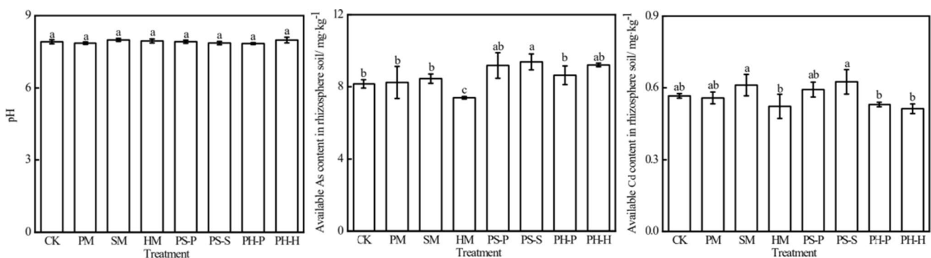
Fig. 2 Soil pH, available As and Cd content in rhizosphere soil after phytoremediation under different treatments
