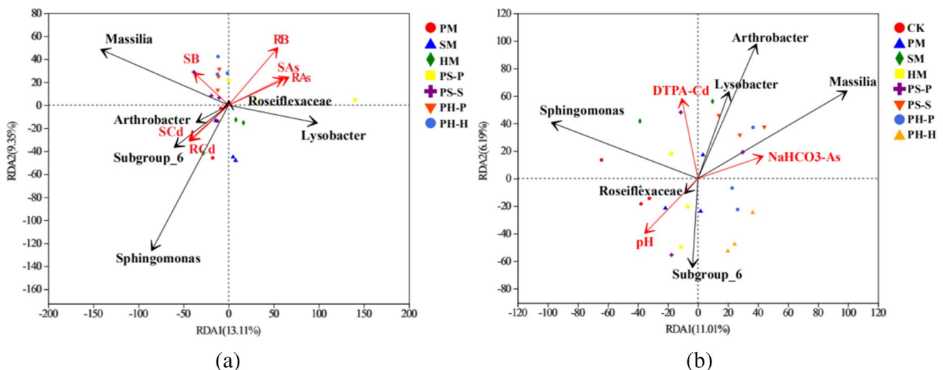
Fig. 4 a Redundancy analysis (RDA) of the soil pH, available As and Cd content, and bacterial communities at genus level. b RDA of the phytoremediation parameters and bacterial communities at genus level. \text{NaHCO}_3\text{-As} , soli available As content; DTPA-Cd, soli avail-
