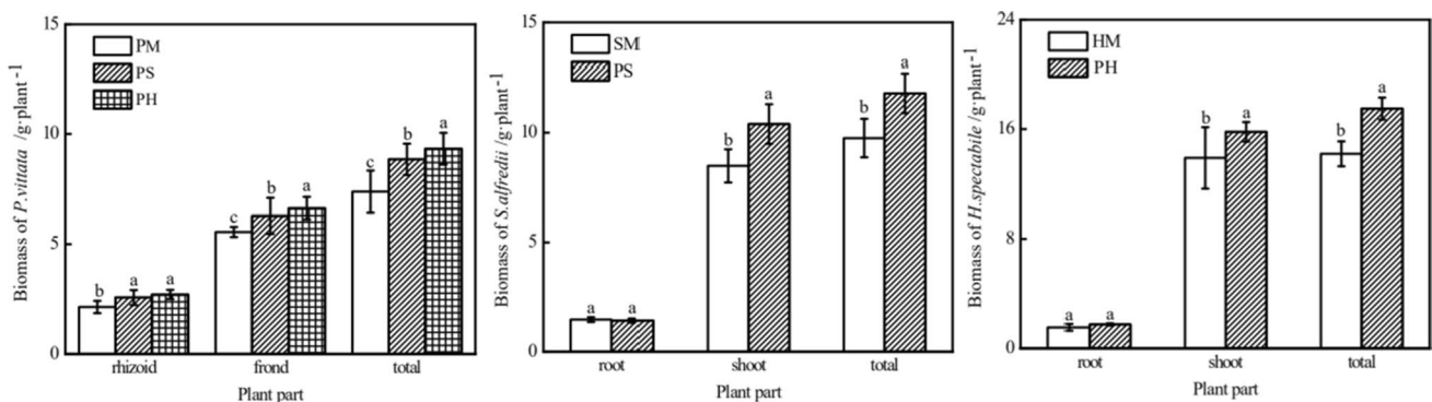
Fig. 1 Biomass of P. vittata , S. alfredii , and H. spectabile under different intercropping systems. PM, P. vittata monoculture; SM, S. alfredii monoculture; HM, H. spectabile monoculture; PS, intercropping of P. vittata and S. alfredii ; PH, intercropping of P. vittata and H. spectabile
