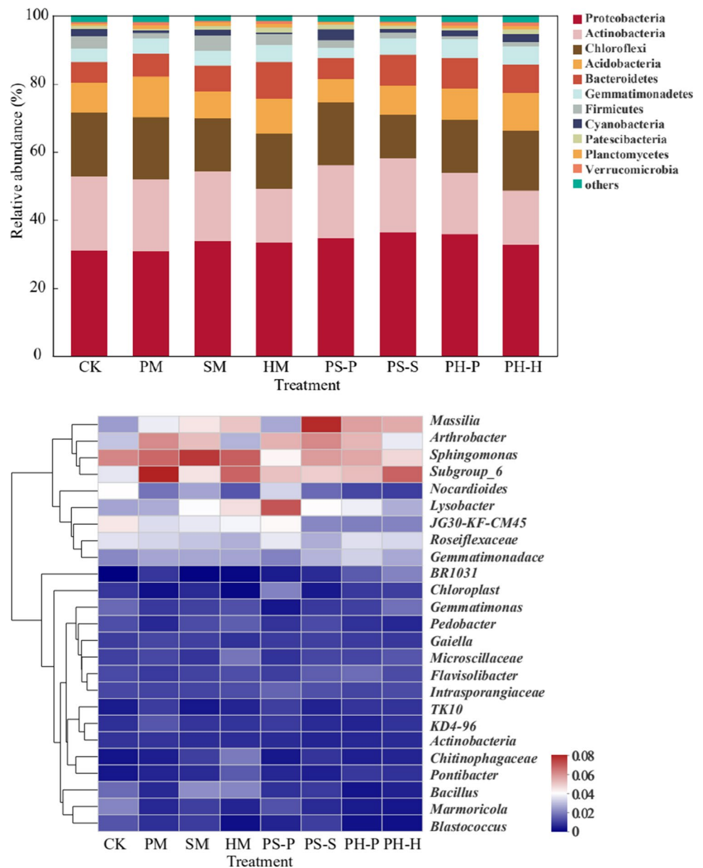
Fig. 3 Soil bacterial taxonomic distribution: relative abundance of predominant phyla (a) and community heatmap analysis at genus level (b) under different treatments
