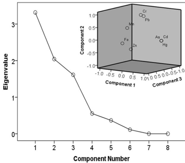
Fig. 3 Principal component analysis of heavy metals by scree plot of the characteristic roots (Eigen values) (inset shows the three-dimensional plot of the PCA loadings demonstrating the relationships among the heavy metals)
