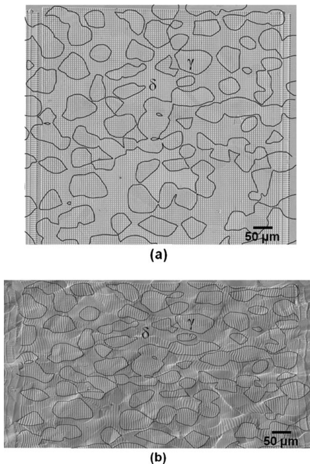
Fig. 3 SEM low magnification-high definition images; (a) before hot deformation; (b) after hot deformation; the contour of the \delta/\gamma interfaces are highlighted with a black line
