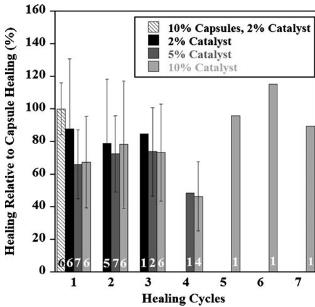
Fig. 9 Healing efficiency relative to the healing of microcapsules beams. The number in each column indicates the number of specimens tested in the average healing value
