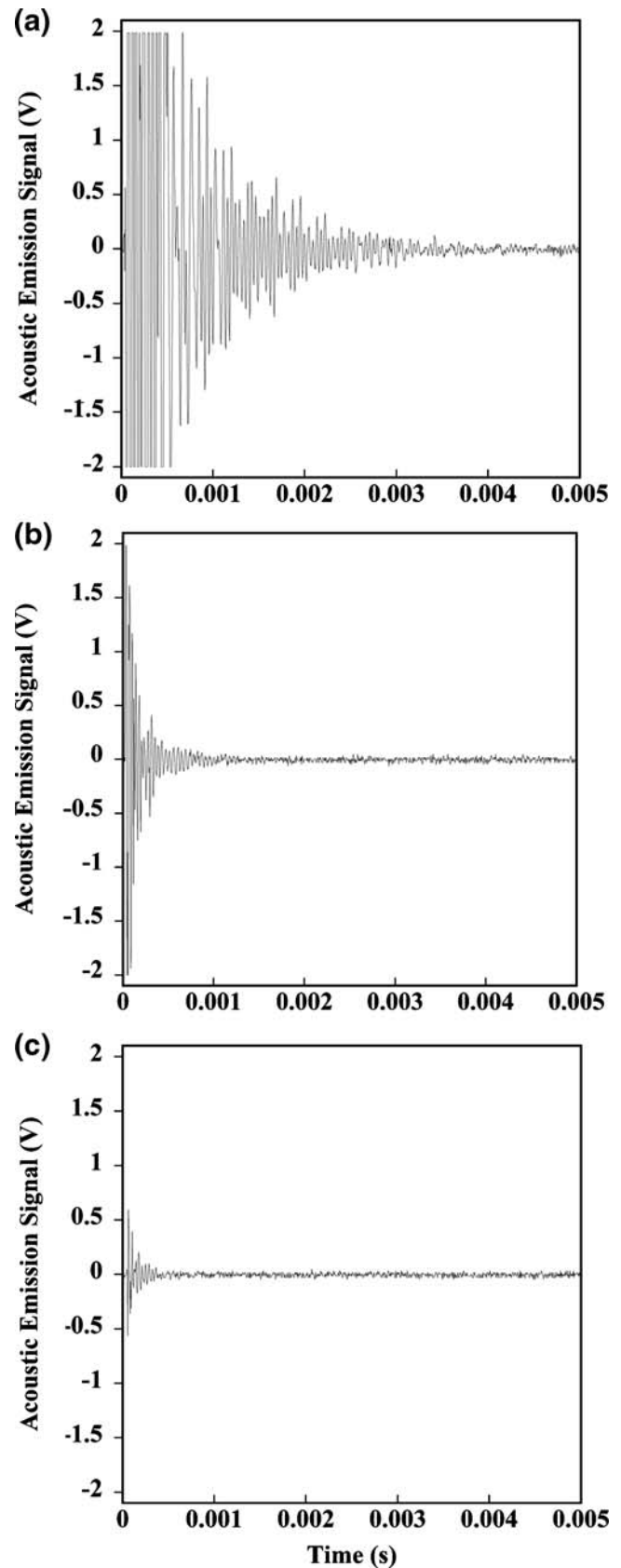
Fig. 4 Representative acoustic emission signals for (a) the formation of a virgin crack, (b) the reopening of a well healed crack, and (c) the reopening of a poorly healed crack
