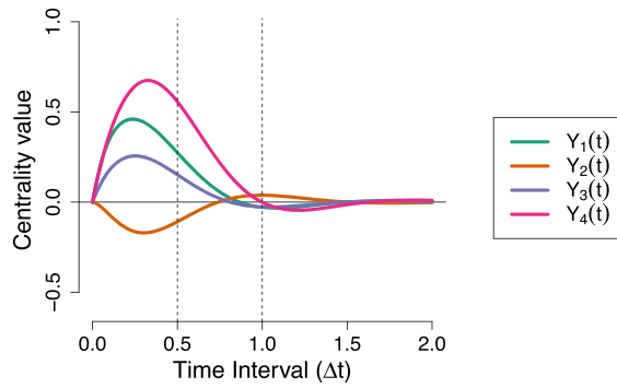
(b) One-Step Expected Influence EI^{(1)}
