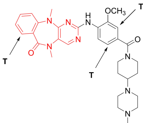
Fig. 2 Chemical structure of [ 3 H]LRRK2-IN-1 (in red: binding moiety; T: possible sites for tritium labeling).
