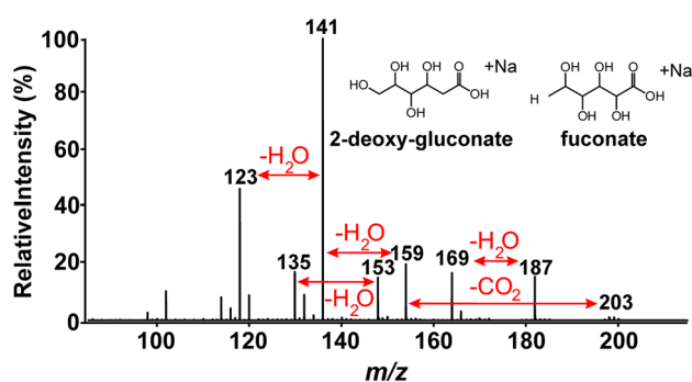
Fig. 4 Direct injection static nESI-MS/MS CID spectrum of m/z 203. Fragment ions at m/z 123, 141, and 159 are consistent with a polyhydroxy carboxylic acid, such as 2-deoxy-gluconate or fuconate ( inset ). A complete assignment of all peaks to the putative structure(s) was not possible, most likely due to selection of multiple isobaric and/or isomeric species prior to dissociation
