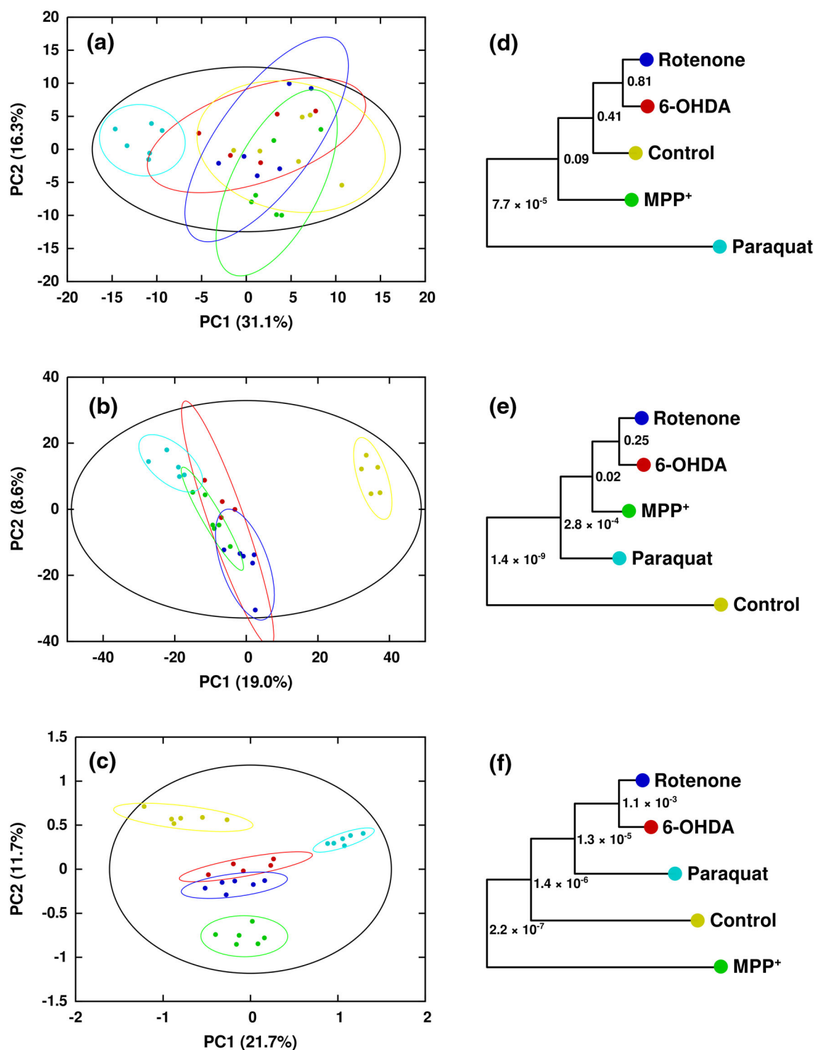
Fig. 2 Scores generated from (a) PCA of 1 H NMR in vacuo, (b) PCA of DI-ESI-MS in vacuo, and (c) MB-PCA of 1 H NMR and DI-ESI-MS. Separations between classes are greatly increased upon combination of the two datasets via MB-PCA. Symbols designate the following classes: Control (yellow circle), Rotenone (blue circle),
