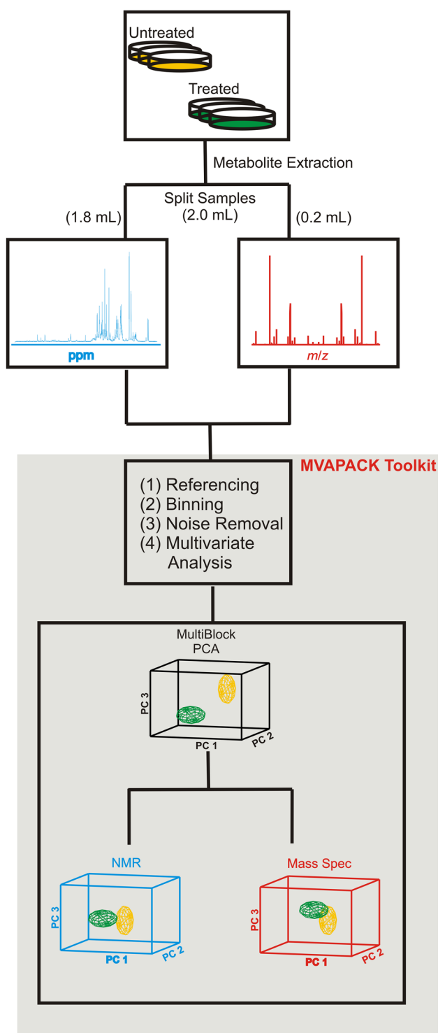
Fig. 1 A flow chart illustrating our protocol for combining NMR and MS datasets for metabolomics. 2.0 mL of a single metabolite extract was split into 1.8 and 0.2 mL for NMR and MS analysis, respectively. Spectral binning of the NMR data used adaptive intelligent binning. First, the background is subtracted from the MS spectrum followed by spectral binning. Spectral binning of the MS data used fixed binning with a set bin width of 0.5 m/z . Baseline noise removal and normalization separately applied to the NMR and MS data sets. The NMR and MS datasets were modeled by MB-PCA and MB-PLS. The resulting block scores and loadings were analyzed for significantly contributing metabolites
