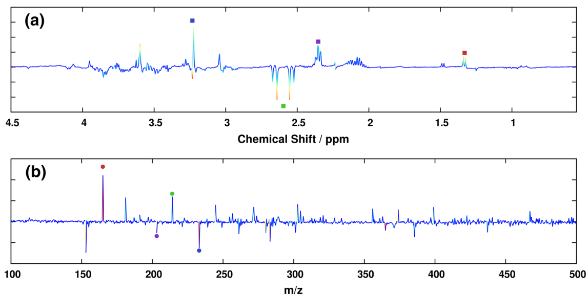
Fig. 3 Backscaled MB-PLS-DA first component loadings generated from (a) the ^1\text{H} NMR block and (b) the DI-ESI-MS block that compare control with drug treatment. The peaks in the loadings are labeled with the same colored symbol ( ^1\text{H} NMR, square; MS, circle) and were assigned to the following metabolites: lactate (red square),
