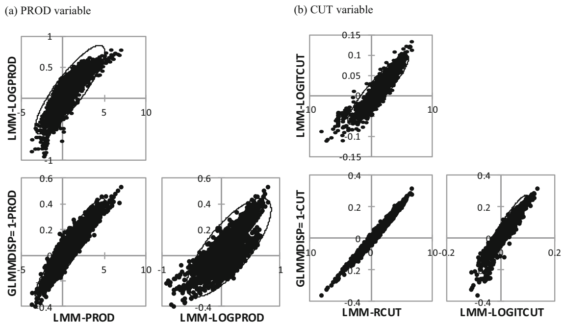
Fig. 1 Correlation between the predicted values obtained with the three different approaches and model (2). X axis — LMM predicted values assessed with linear mixed model and original variable; LMM-LOG and LMM-LOGIT predicted values assessed with linear mixed model and
