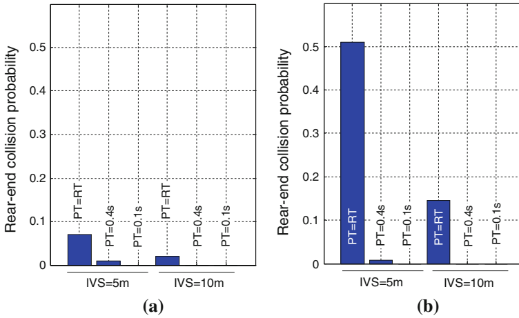
Fig. 6 Rear-end collision probability when dimensioning V2V communications protocols based solely on the avoidance of intersection collisions, i.e. with a transmission power so that the probability of not receiving a CAM before CD is equal to 0.01 for v = 70 \text{ km/h} , N = 2 and 100 Bytes payload. a RT = 0.75 \text{ s} . b RT = 1.5 \text{ s}
