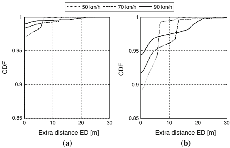
Fig. 10 Cumulative Distribution Function of ED estimated in realistic urban SUMO scenarios. PT = RT = 0.75 s. a Vehicular density D1. b Vehicular density D2
