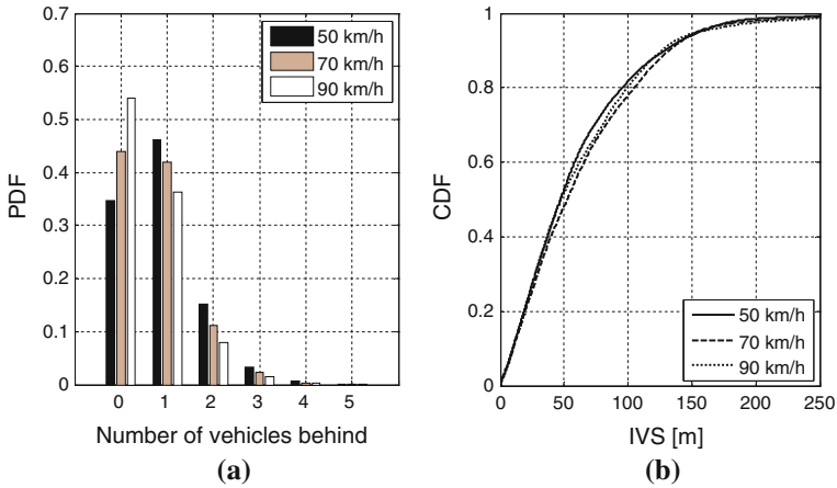
Fig. 9 Impact of realistic SUMO mobility scenarios on the number of vehicles and inter-vehicle distances with traffic density D2. a PDF of number of vehicles behind the lead vehicle in the chain. b CDF of inter-vehicle distances
