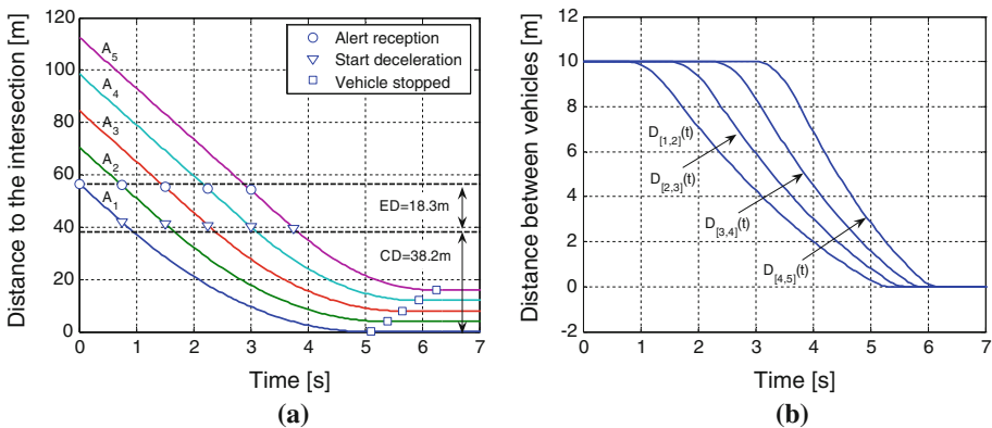
Fig. 3 Illustration of the distance to the intersection and distance between vehicles considering the proposed methodology. Case: RT = PT = 0.75 s, v = 70 km/h, IVS = 10 m, L_n = 4 m, N = 5 vehicles. a Distance to the intersection. b Distance between vehicles
