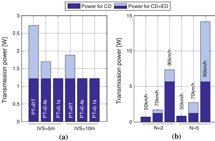
Fig. 7 Required transmission power to exchange at least one CAM before CD and before CD + ED with probability p = 0.9999 considering 100 Bytes payload. a v = 70 \text{ km/h} , N = 2 vehicles and RT = 0.75 \text{ s} . b IVS = 5 \text{ m} , RT = 0.75 \text{ s} and PT = 0.4 \text{ s}
