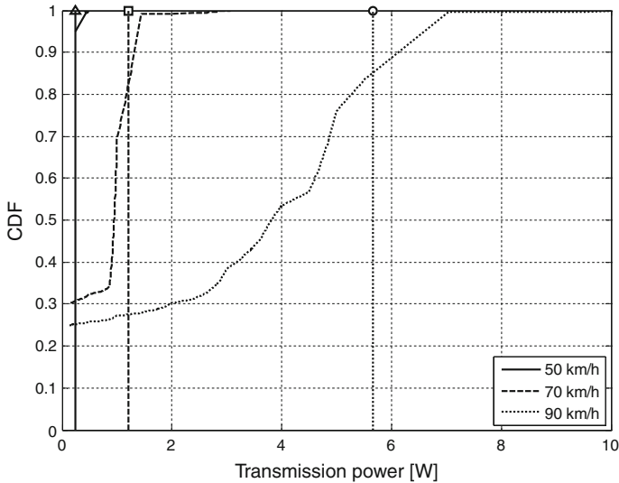
Fig. 11 Cumulative Distribution Function of the transmission power needed to receive the first broadcast message before CD + ED for a target p = 0.9999 using SUMO with traffic density D2 and RT = PT = 0.75 s
