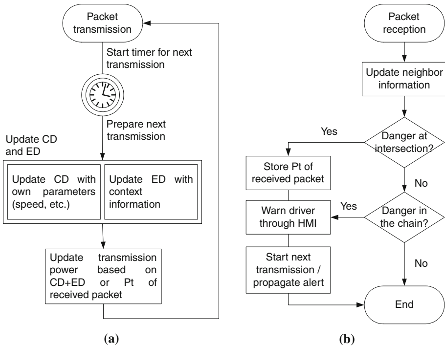
Fig. 2 Flow chart for the transmission and reception of CAM messages in the case of the proposed context-aware approach. a Transmission process. b Reception process
