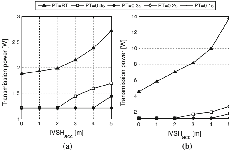
Fig. 8 Required transmission power to exchange at least one CAM before CD and before CD + ED with probability p = 0.9999 considering realistic positioning for IVS_m = 10 m, RT = 0.75 s, v = 70 km/h and 100 Bytes payload. a N = 2 . b N = 5
