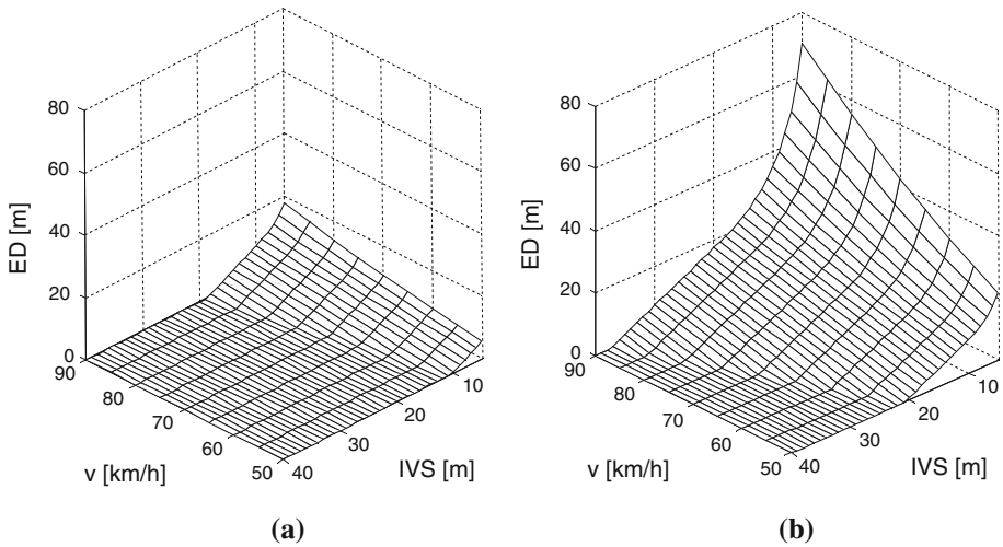
Fig. 4 Extra distance as a function of the vehicular speed and the IVS distance for N = 2 vehicles. a RT = PT = 0.75 s. b RT = PT = 1.5 s
