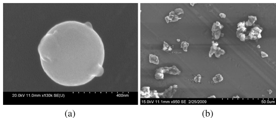
Fig. 10 Scanning electron microscope images from MOUDI stages with cutpoint particle diameter of a 0.32 \mu\text{m} , particle depicted was identified to contain 21.19 \pm 4.45\% Pb by weight by electron dispersive spectroscopy and b 6.1 \mu\text{m}
