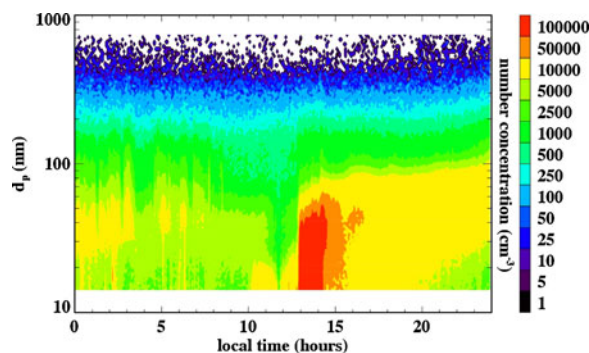
Fig. 12 A full day of size distribution data (SMPS measurements for April 18, 2009). Note the relatively high concentrations of 14–50 nm particles, starting at 1 pm
