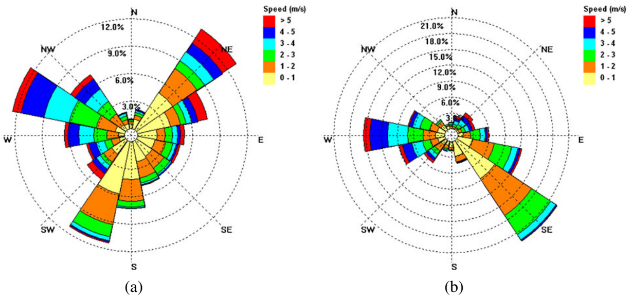
Fig. 14 Wind roses from two weather stations located within 2 miles of each other for December 2008 through November 2009: a Winkelman, where the MOUDI is located, and b
