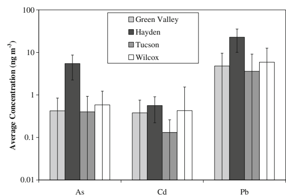
Fig. 2 Comparisons of As, Cd, and Pb content in atmospheric air (TSP samples). Values are averages over ten 24-h sampling periods at various sites in Southeast Arizona from July to December 2009. Error bars represent standard deviations over the ten sampling periods
