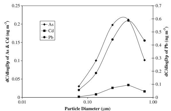
Fig. 8 Log-normal plot of lead, arsenic, and cadmium concentrations for particle diameters <1 µm in MOUDI samples taken at the Hayden site for a 96-h sampling period starting on October 14, 2009 (Fig. 6). From these results, the calculated mean diameter is 0.17 µm, and the geometric standard deviation is 2.68
