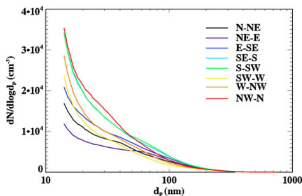
Fig. 13 Aerosol number size distributions as a function of wind direction for the measurement period March 17 through May 20, 2009
