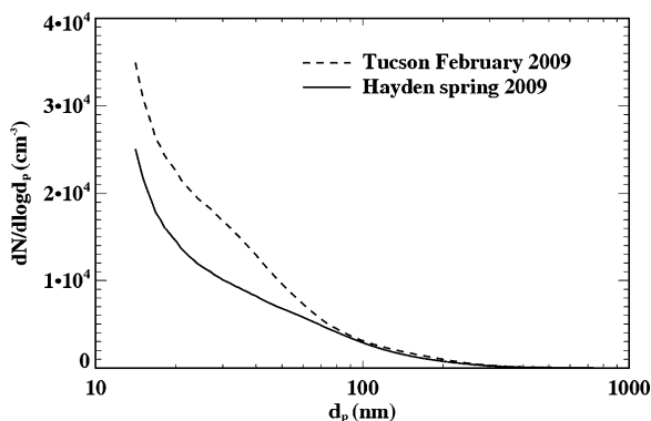
Fig. 11 Average SMPS size distribution over one MOUDI measurement period (March 17 through May 20, 2009) compared with an average (February 25 through March 13, 2009) from the city of Tucson
