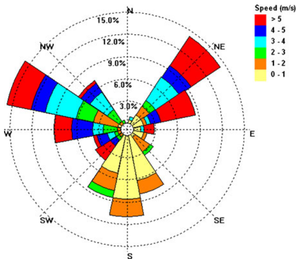
Fig. 9 Wind rose obtained from the weather station co-located with the MOUDI sampler for the 96-h sampling period starting on October 14, 2009 (corresponding to data in Figs. 6, 7, and 8). The results show a relatively high frequency of high wind speeds ( >3 m/s) from the WNW direction, which corresponds with the orientation of the mine tailings with respect to the sampler
