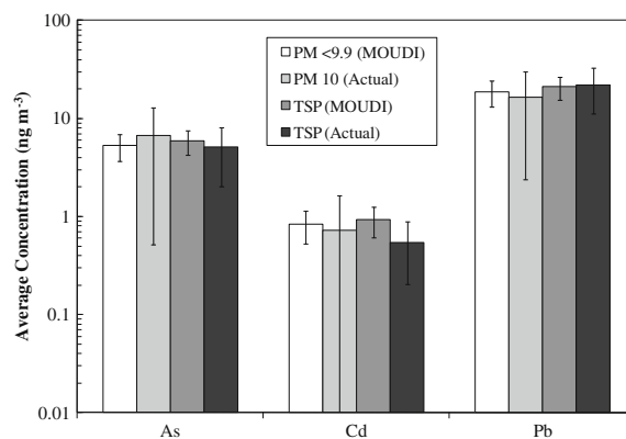
Fig. 4 Comparisons of metal and metalloid content of MOUDI samples with \text{PM}_{10} data from EPA and TSP observations at the Hayden site. Samples were taken between December 2008 and November 2009 for 36 and 55 sampling periods for the MOUDI and \text{PM}_{10} monitor, respectively. The TSP concentrations were averaged for 18 sampling periods spanning July 2009 to March 2010. Sampling periods may not have occurred on the exact same days. For MOUDI samples, \text{PM}_{9,9} represents the average of the summed mass concentrations in the corresponding size range, and TSP represents the average total concentration
