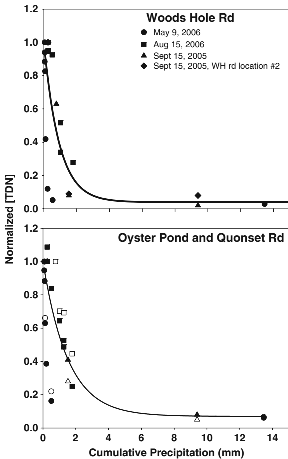
Fig. 3 Normalized total dissolved nitrogen (TDN) concentrations as a function of cumulative precipitation during three storm events on Woods Hole Road ( top panel ) and Oyster Pond and Quonset Roads ( lower panel —symbols in the lower panel represent the same dates as indicated in the upper panel; open symbols are for Quonset Road and closed symbols are for Oyster Pond Road). The equations for the regressions are: Upper panel : Y = 0.04 + 0.96 \cdot \exp(-1.06 \cdot X) , R^2 = 0.59 , p = 0.0005 ; Lower panel : Y = 0.07 + 0.93 \cdot \exp(-0.66 \cdot X) , R^2 = 0.58 , p < 0.0001
