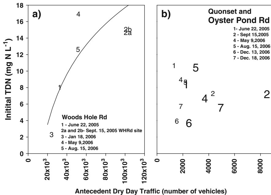
Fig. 2 a Initial total dissolved nitrogen (TDN) concentrations in road runoff for Woods Hole Road as a function of antecedent dry day traffic (ADDT) estimates for five rainfall events. Each data point is plotted with a number, which also serves as a code for the sampling date, as indicated. The two sampling stations on Woods Hole Road for Sept 15, 2005 ( a and b ) were averaged prior to the
