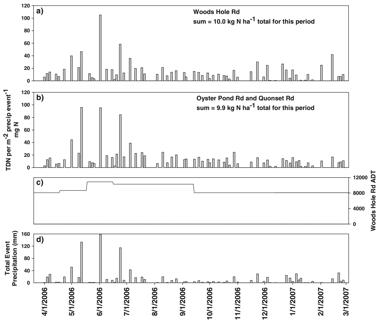
Fig. 4 Calculated total dissolved nitrogen (TDN) in road runoff for each precipitation event for a Woods Hole Road, b Oyster Pond Road and Quonset Road combined, c the monthly
