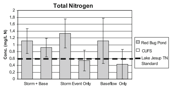
Fig. 7 Storm event and baseflow comparison for TN
