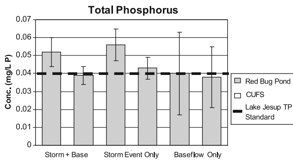
Fig. 6 Storm event and baseflow comparison for TP
