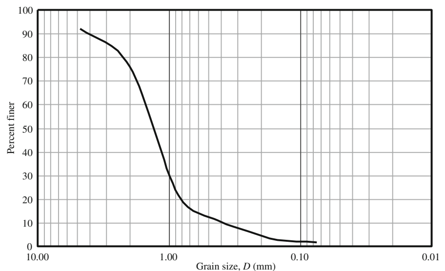
Fig. 4 Graduation curve for particle size distribution
