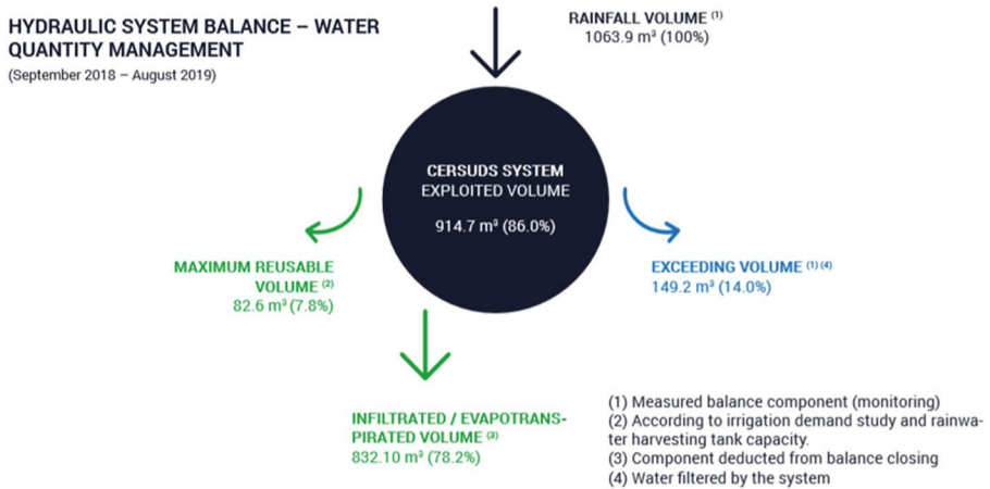
Fig. 8 Volumetric balance of the system for the period September 2018—August 2019 (LIFE CERSUDS 2019)
