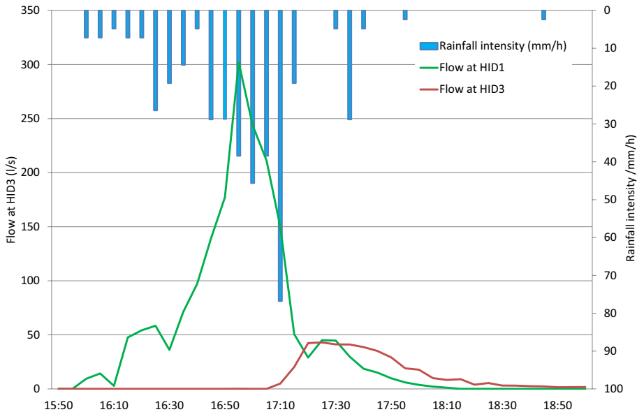
Fig. 9 Hyetograph and hydrographs for the rainfall event registered on 18 Oct 2018
