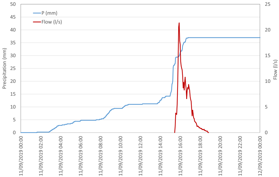
Fig. 10 Hyetograph and hydrograph for the rainfall event registered on 11 Sep 2019
