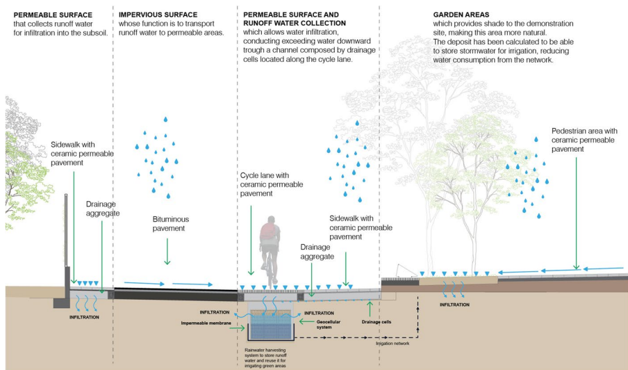
Fig. 5 Scheme of the sustainable drainage system performed in Benicàssim (LIFE CERSUDS 2019)
