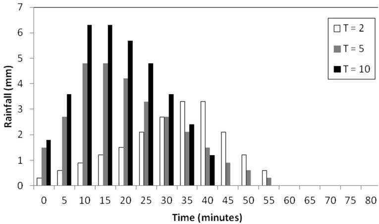
Fig. 1 Hyetographs for the T=2, 5 and 10 return period events. Total rainfall is 19.8 mm for T=2, 29.4 mm for T=5 and 35.7 mm for T=10.
