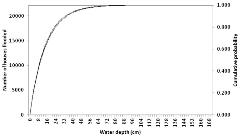
Fig. 5 Number of properties flooded by water depth for the 1a scenario (Table 1) Dashed lines indicate 95 % confidence limits.
