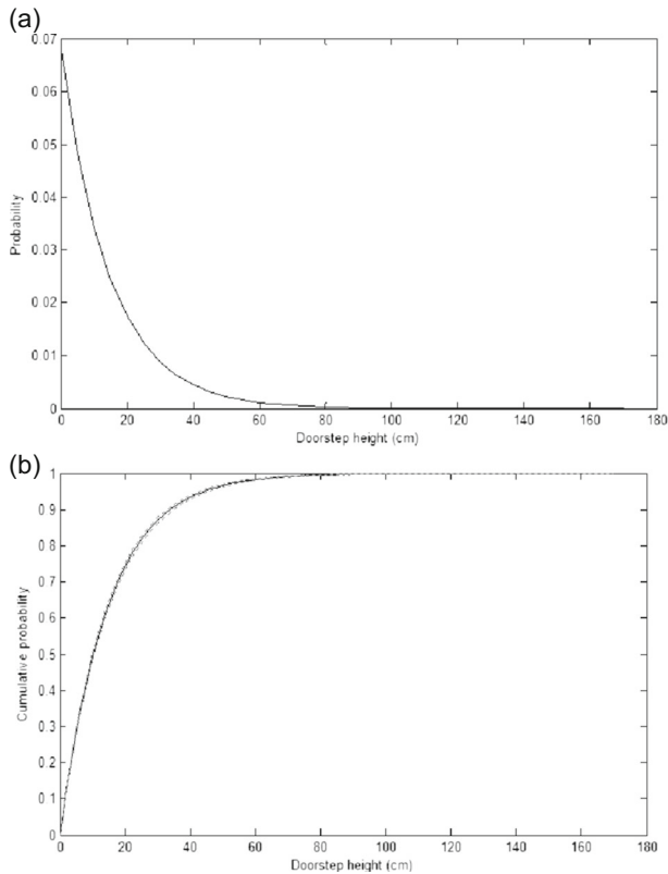
Fig. 3 a Probability- and b Cumulative-density functions (PDF; CDF respectively) of the Rotterdam doorstep measurements.
