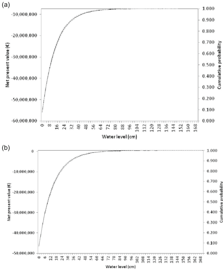
Fig. 7 Net-present value of the risk reduction measures for a the disconnection and Gender measures combined (the ‘b’ scenarios) and b the disconnection measure only (the ‘c’ scenarios). See Table 1 for scenario details. Dashed lines indicate 95 % confidence limits.
