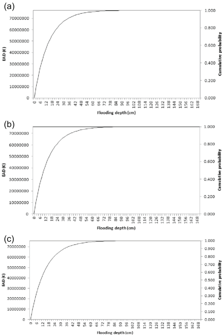
Fig. 6 EAD distribution for a the ‘a’ scenarios; b the ‘b’ scenarios and; c the ‘c’ scenarios. See Table 1 for scenario definitions.
