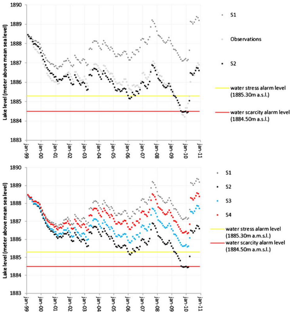
Fig. 5 top: Simulated lake and levels for the recent period with ‘natural’ conditions (S1) and ‘including abstractions’ (S2); bottom: Lake levels influenced by groundwater abstractions and surface water abstractions for four different situations: a natural situation (S1), a situation with all abstractions (S2), a situation with no groundwater abstractions (S3), a situation with no surface water abstractions (S4)
