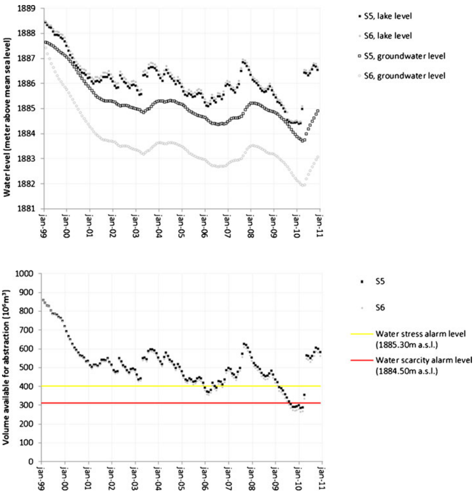
Fig. 6 top: Simulated lake levels and groundwater levels for the recent period (1999–2010) with all the abstracted water obtained from the lake directly (S5) and all the abstracted water obtained from the lake aquifer (S6); bottom: Water volumes for the period 1999–2010 done for different simulations: Lake volumes for a situation in which all abstractions are obtained from the lake directly (S5); Total available volume for a situation in which all abstractions are obtained from the aquifer (S6). For S6 water availability equals lake volume minus the difference between aquifer volumes for S5 and S6
