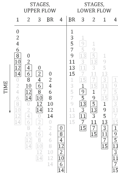
Figure 35 Timing of a 16-point 2-parallel radix-2 M 2 DF FFT architecture.
