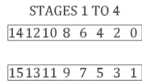
Figure 31 Timing of a 16-point 2-parallel radix-2 MDF FFT architecture.
