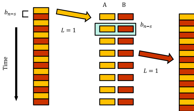
Figure 28 Timing of a radix-2 SC FFT architecture.
