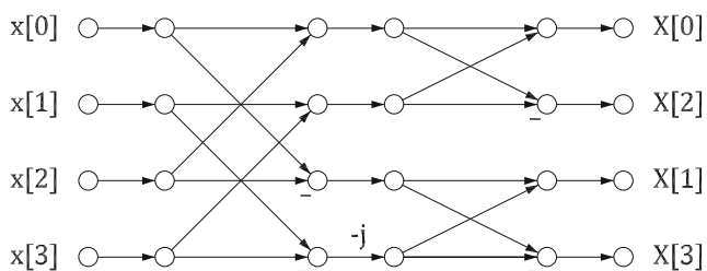
Figure 4 Radix-4 butterfly.
