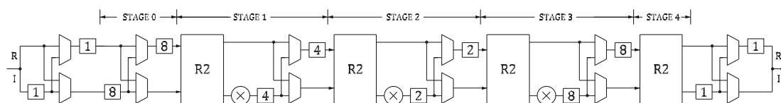
Figure 23 16-point radix-2 SDC FFT architecture that divides the data in real and imaginary parts.
