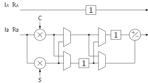
Figure 24 Alternative rotator in a radix-2 SDC FFT architecture that divides the data in real and imaginary parts.
