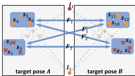
Fig. 7 A scene with 2 lights and 3 casters. In each pose, fundamental matrices enable us to split the 6 shadows into 2 sets (blue rectangles) of 3 shadows, each set corresponding to one of the lights. However, the fundamental matrices cannot match these shadow sets across poses due to an ambiguity that allows connecting any pair of sets (blue arrows) (Color figure online)
