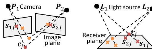
Fig. 4 Cameras versus point lights. A camera matrix P_i projects a scene point c_j to an image point s_{ij} just like a light matrix L_i projects a scene point c_j to a shadow s_{ij} . Conventional SfM estimates P_i and c_j from \{s_{ij}\} and in this paper we show how to estimate L_i and c_j from \{s_{ij}\}
