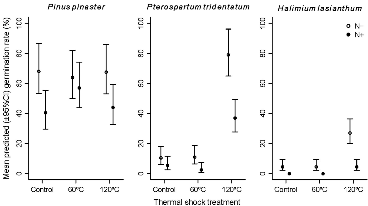
Fig. 1 Model predicted values (mean ± 95% confidence intervals) of the seed germination rate (%) of P. pinaster , P. tridentatum and H. lasianthum after the thermal shock [control
