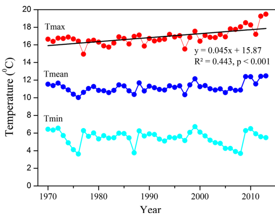
Fig. 2 Annual temperature trend of Thakmarpha (Mustang); maximum temperature ( T_{max} ), mean temperature ( T_{mean} ), and minimum temperature ( T_{min} )
