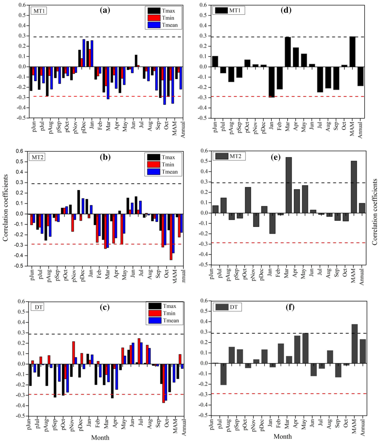
Fig. 5 Correlation coefficients of tree ring width indices, with total monthly maximum ( T_{max} ), mean ( T_{mean} ), and minimum temperature ( T_{min} ); MT1 (a), MT2 (b), DT (c), and total monthly rainfall; MT1 (d), MT2 (e), DT (f); of June in the
