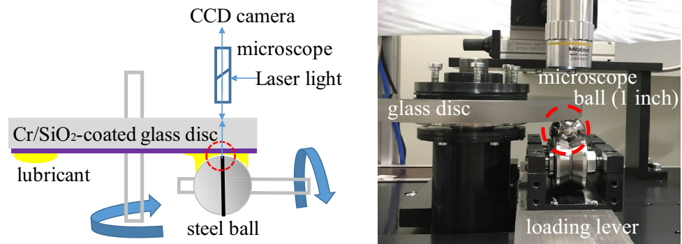
Fig. 2 Optical ball-on-disc test rig for lubricating film thickness measurement, left: diagrammatic drawing; right: photo of the ball-on-disc test rig at Leibniz University Hannover
