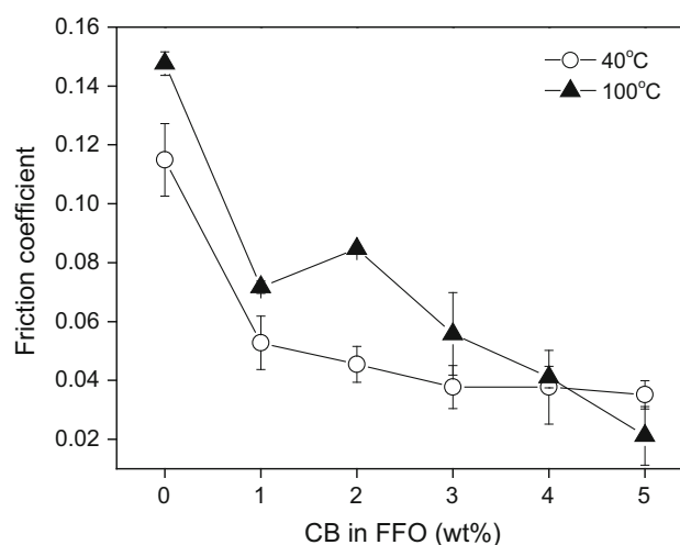
Fig. 4 Friction as a function of soot content in FFO. The friction values are an average of friction coefficient during the last 30 min of tests
