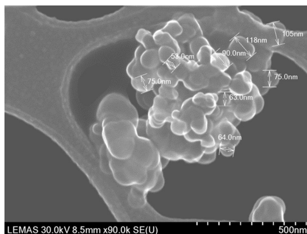
Fig. 1 STEM micrograph of carbon black particles
