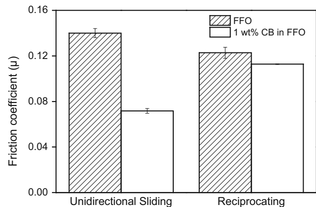
Fig. 5 Friction comparison at different sliding configurations
