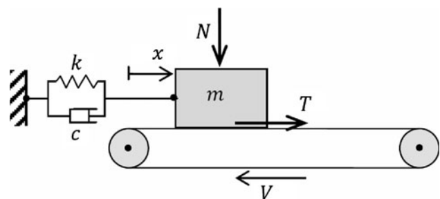
Fig. 1 Friction-induced vibration of a mass spring oscillator
