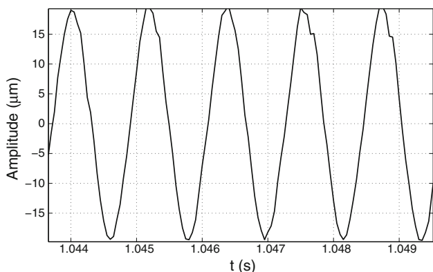
Fig. 11 Vibration of sample A blade
