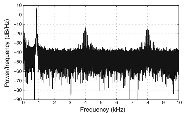
Fig. 12 Power spectral density of the vibration signal of sample A
