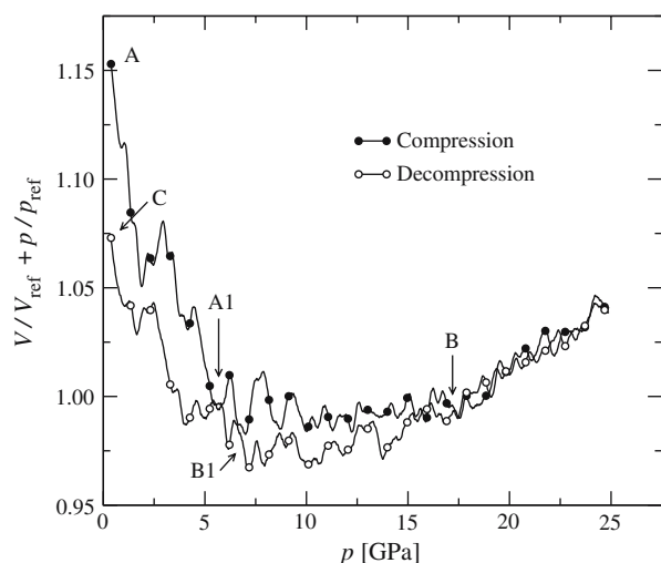
Figure 1. Instantaneous normalized volume, V/V_{\text{ref}} + p/p_{\text{ref}} as a function of pressure, p , for the zinc phosphates. V_{\text{ref}} = 200 \text{ cm}^3/\text{mol} and p_{\text{ref}} = 80 \text{ GPa} . Key points along the plot are denoted with the labels A through C and are discussed in the main text. The representation of the data as V/V_{\text{ref}} + p/p_{\text{ref}} against p , instead of V against p , was performed to keep the plotted data in a narrow range. The bulk modulus, B , can be approximated in units of GPa as B = (-\text{local slope} + 1/80)^{-1} .
