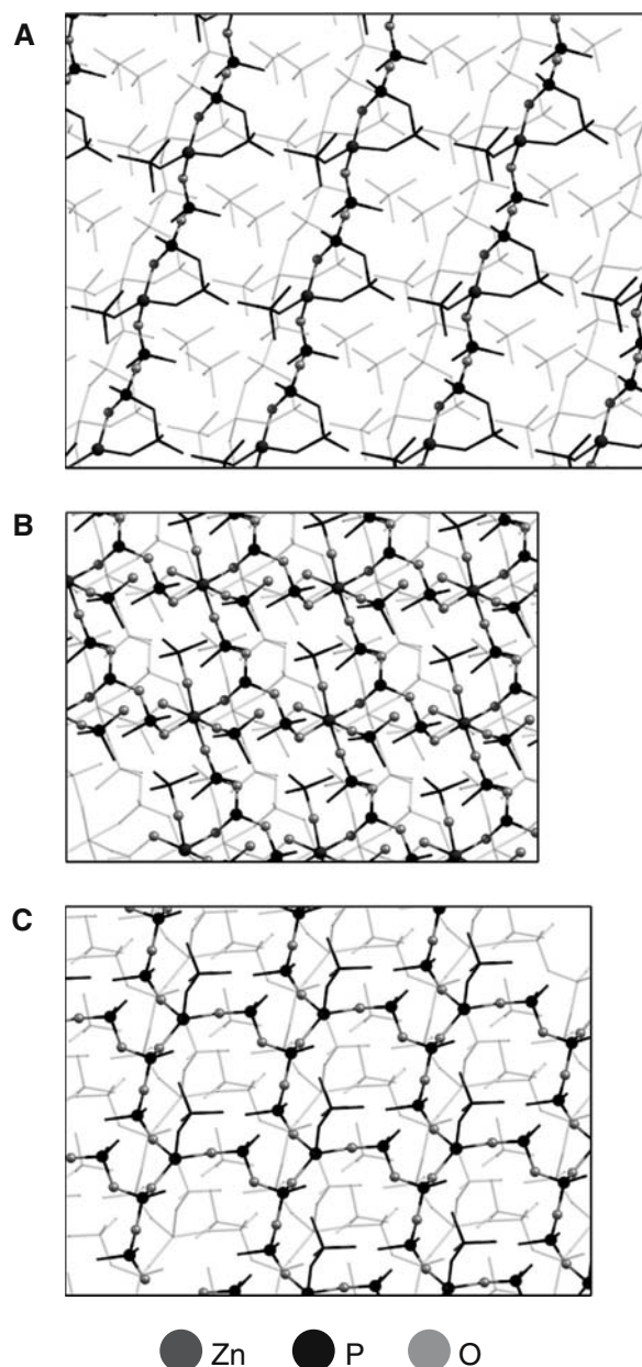
Figure 2. Representative structures of the system observed during the simulation. (A) The initial structure. (B) The structure with hexacoordinate Zn observed above 17 \text{ GPa} . (C) The final structure of the c/d cycle. In all cases the simulation cell is shown repeated periodically. Atoms involved in extended bonding are denoted with a ball-and-stick representation. Atoms in underlying layers are faded out to aid in visualization. Hydrogen atoms have been omitted for clarity.
