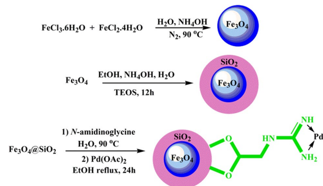
Scheme 1 Procedure for preparation of the \text{Fe}_3\text{O}_4@ \text{SiO}_2@ \text{N} -amidinoglycine@Pd 0 Catalyst
