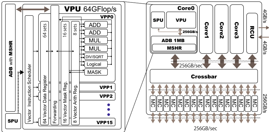
Fig. 2 SX-ACE processor
