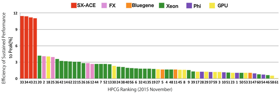
Fig. 22 HPCG efficiency ranking
