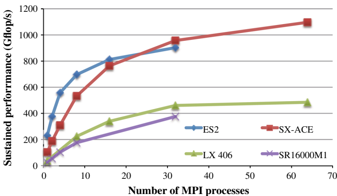
Fig. 18 Performance of hybrid parallelization
