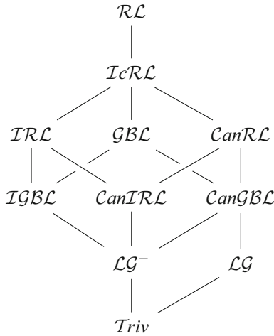
Figure 1. Varieties of integrally closed residuated lattices
