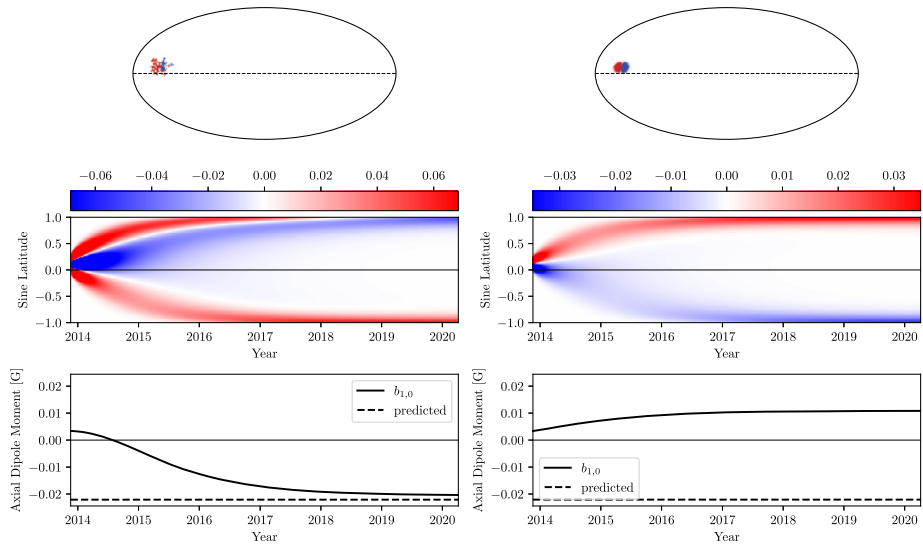
Fig. 8 Evolution of an active region with asymmetric bipolar shape, taken from the simulation in Fig. 1. The left column shows the region with its observed shape, with second row showing \langle B_r \rangle and third row the axial dipole strength b_{1,0} . The right column shows the evolution of an “equivalent” symmetric BMR having the same initial flux and b_{1,0} . The dashed line shows the final b_{1,0} predicted by equation (36) using the observed magnetogram
