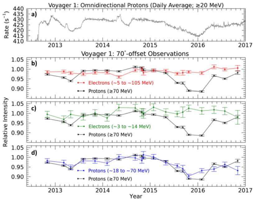
Fig. 21 Observations from CRS on VI reveal a species dependence in the episodes of GCR anisotropy. (a) the HET1 omnidirectional ( \gtrsim 20 MeV; grey) and (b–d) bi-directional protons ( \gtrsim 70 MeV; black) show prominent decreases in intensity when the telescope fields of view overlap with 90^\circ pitch angles during 70^\circ -offset re-pointing maneuvers. (d) A clear signature is also evident in low-energy protons ( \sim 18 to \sim 70 MeV; blue). In contrast, (c) neither low-energy electrons ( \sim 3 to \sim 14 MeV; green), nor (b) those of similar energy ( \sim 5 to \sim 105 MeV) exhibit much of a response, implying that the effect cannot be attributed to energy dependence. Moreover, the protons of (c) and electrons of (d) are viewed on the same telescope, while the electrons of (b) are recorded by a telescope that is more directly aligned with 90^\circ pitch angle, so the differences cannot be simply explained by viewing direction. Figure from Rankin et al. (2020)
