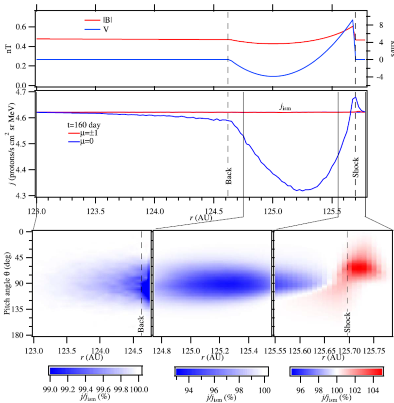
Fig. 27 Radial profiles of the magnetic field strength, plasma speed, intensity of 100 MeV GCR protons and pitch-angle distribution proposed by a weak pressure pulse in the VLISM. Detailed variations of the pitch-angle distribution are shown in three segments with different radial distance and magnitude scales. The GMIR propagates radially at 40 km/s and has a thickness of 1.06 AU. Figure from Zhang and Pogorelov (2020)
