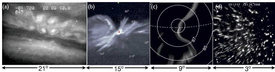
Fig. 3 Ground-observations of fine scale auroral phenomena with fields-of-view as shown: a ) Auroral curls (Vogt et al. 1999), b ) “Flaming” auroral filaments (Dahlgren et al. 2013), c ) Auroral “packets” (Semeter et al. 2008), d ) Decameter filaments produced by HAARP (Kendall et al. 2010)
