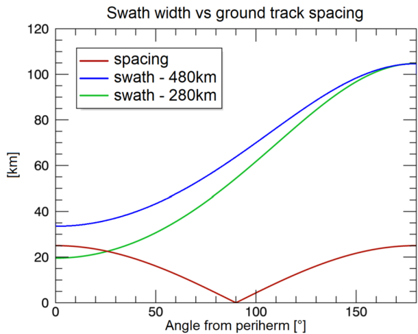
Fig. 5 MERTIS swath width and track to track spacing (red) vs angle from perihelion during the high-resolution mapping phase, assuming perihelion at 280 km (green) and 480 km (blue). Notice that for perihelion at 280 km, the swath width is smaller than the track spacing below 30° from perihelion
