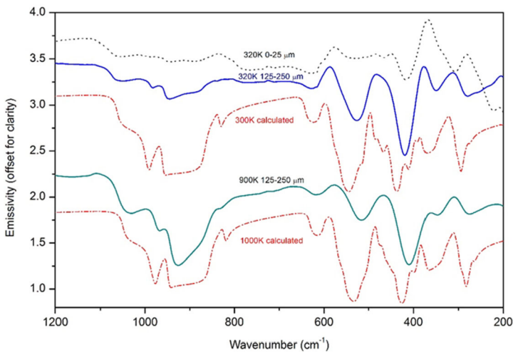
Fig. 14 Comparison between emissivity mid IR spectra (calculated as 1-R) and experimental emissivity measurements. Solid line: Experimental thermal emissivity spectra of \text{Fo}_{89} measured at 320 K and 900 K (extreme situations). Dotted lines: Calculated IR reflectance (inverted) bands of an \text{Mg}_2\text{SiO}_4 ( \text{Fo}_{100} ) end-member. Spectra are offset for clarity
