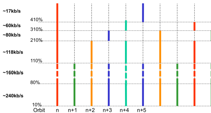
Fig. 7 Schematic display of the operational sequence over a period of 10 orbits
