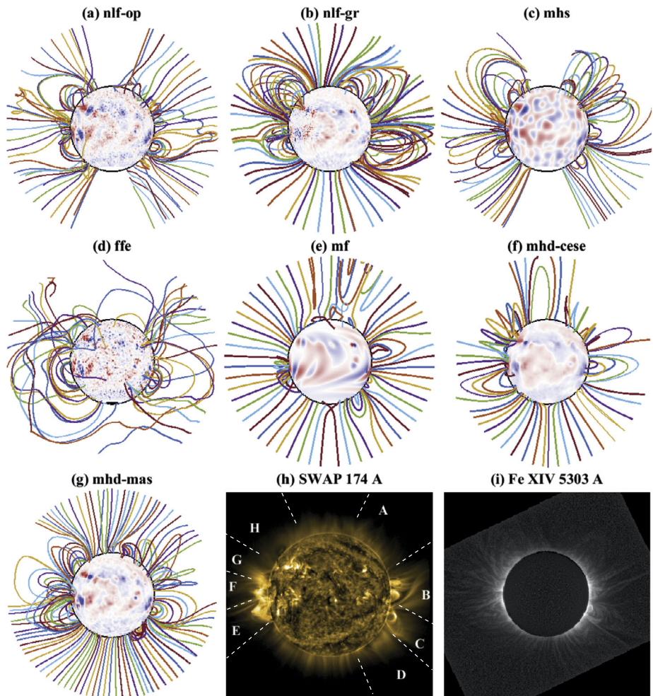
Fig. 7 Magnetic field structure of each model in the plane-of-sky, as viewed from the Earth at the (approximate) eclipse time. (The density of magnetic field lines is arbitrary, and does not correspond to field strength.) Red/blue shading shows B_r at r = R_\odot (saturated at \pm 50 G). Panel (h) shows an EUV 174 Å image of the real corona from PROBA2/SWAP (with median stacking and stray-light correction as described by Seaton et al. 2013). Panel (i) shows an image of the corona in the Fe XIV 5305 Å line from the Habbal eclipse expedition, processed by the MGN algorithm of Morgan and Druckmüller (2014) (with parameter h = 0.9 ) to bring out the streamer structure. Several angular regions are labelled in panel (h) for ease of reference in the text
