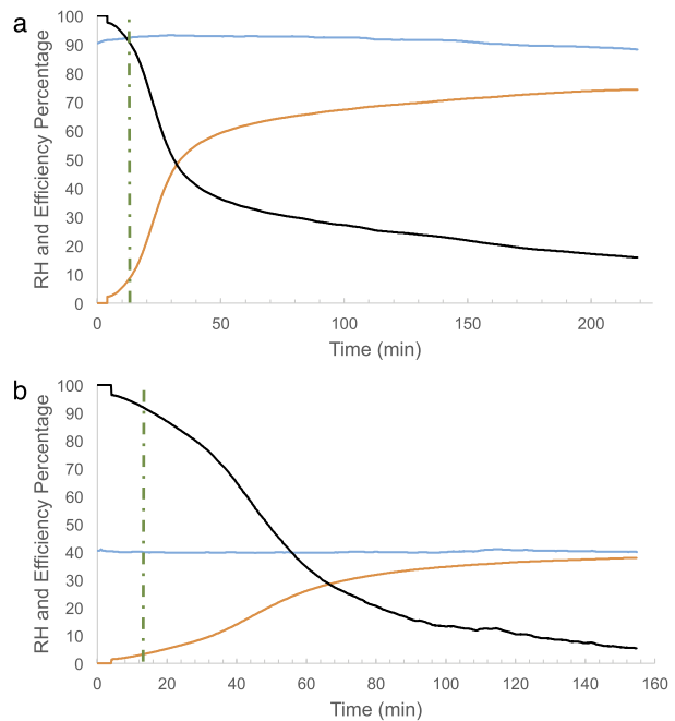
Fig. 25 SRC filter performance for the 90% (top) and 40% (bottom) humidity tests. The blue lines are the inlet humidity, orange is the outlet humidity, and black is the filter efficiency. Vertical dashed green line at 13.3 min corresponds to 20 liters of air passing through the filter
