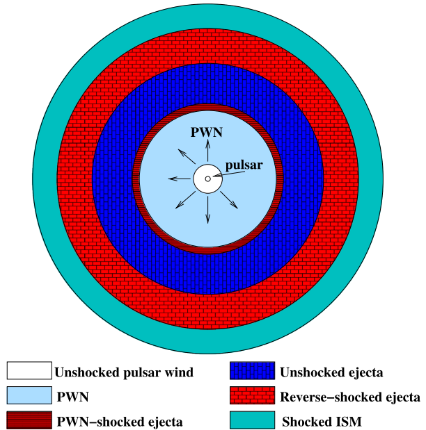
Fig. 1 Cartoon of PWN inside a shell SNR. The SNR blast wave is the outermost circle
