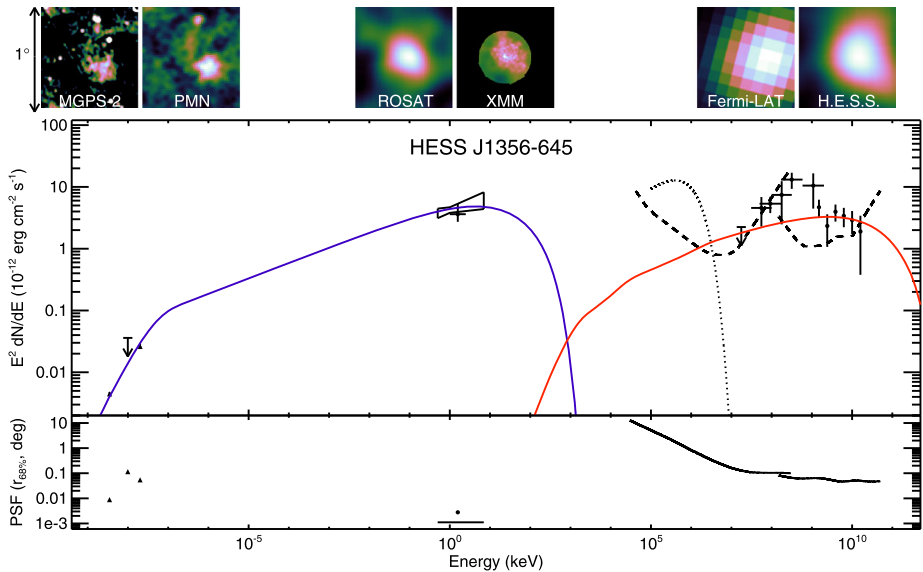
Fig. 38 Broadband spectrum of the PWN HESS J1356-645 (H.E.S.S. Collaboration et al. 2011; Ackermann et al. 2016). The blue and red solid curves give the SC and IC emission from a one-zone, time-independent, modeling performed in H.E.S.S. Collaboration et al. (2011). The dotted line represents the best-fit phase-averaged spectrum of PSR J1357-6429 as obtained in Lemoine-Goumard et al. (2011). The two dashed lines show the Fermi-LAT and H.E.S.S. point-source sensitivities (see text for more details). The 1^\circ -wide multi-wavelength images, as obtained in H.E.S.S. Collaboration et al. (2011), Ackermann et al. (2016), centered on the PSR position, are also shown. The lower panel presents the angular resolutions of the considered radio, X-ray and gamma-ray instruments
