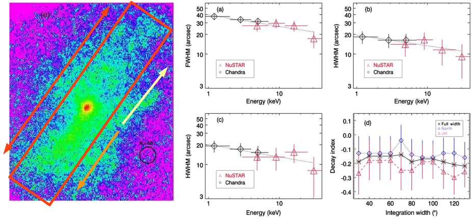
Fig. 19 Left: Box used to extract profiles from NuSTAR image of MSH 15-52. Profiles were summed along the minor dimension (100''), and extents as a function of energy displayed in panels to the right . Panel (a): FWHM of profiles centered on the pulsar extending in both directions. (b): Extending from the pulsar to the NW. (c) Extending from the pulsar to the SE (along the jet). (d) Energy shrinkage ("decay") indices m (with extents \propto E^m ). Plots from An et al. (2014)
