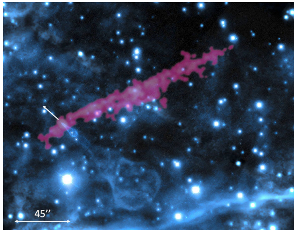
Fig. 29 Smoothed X-ray image from Fig. 28 overlaid onto the H\alpha image showing the Guitar. The H\alpha image is taken from http://chandra.harvard.edu/photo/2015/archives/
