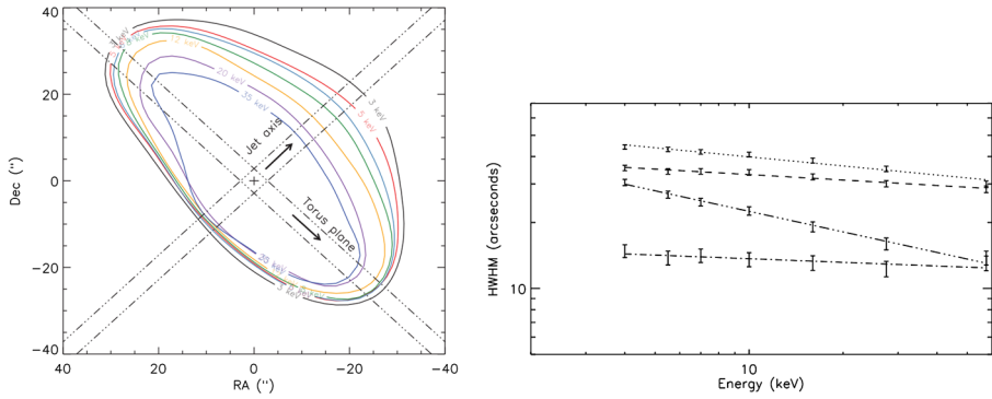
Fig. 11 Left: Crab 50% peak intensity contours at different energies (Madsen et al. 2015). From outside in, 3–5, 5–6, 6–8, 8–12, 12–20, 20–35, and 35–78 keV. Right: Fits to the HWHM along different directions. From top to bottom: NE torus plane, SW torus plane, NW jet axis, and SE jet axis
