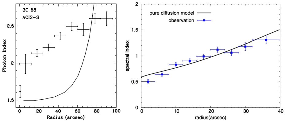
Fig. 21 Left: Observed photon index \Gamma as a function of radius in 3C 58 (Slane et al. 2004). Curve: Prediction from Kennel–Coroniti pure-MHD spherical advection model (Reynolds 2003). Right: Diffusion model for G21.5-0.9 (Tang and Chevalier 2012, data from Slane et al. (2000))
