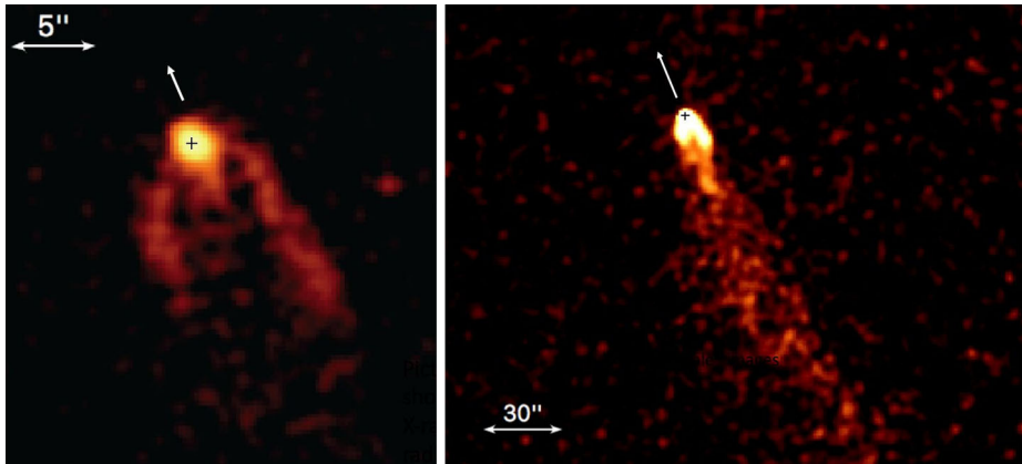
Fig. 31 Left: Compact X-ray nebula in the vicinity of PSR J1509-5850. Right: ACIS image demonstrating the transition from the compact nebula to the southwest tail
