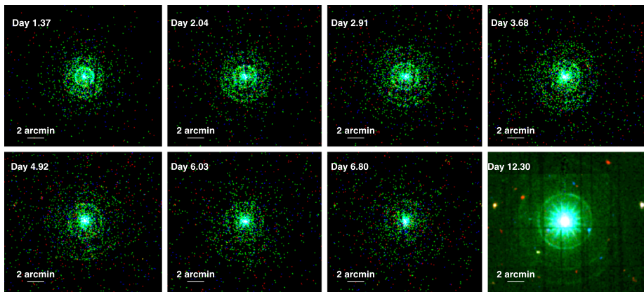
Fig. 43 Images of the expanding X-ray rings caused by interstellar dust scattering around the transient magnetar 1E 1547.0-5408 (from Tiengo et al. 2010b). The seven Swift observations and the XMM-Newton observation (bottom right panel) were obtained from one to 12 days after a very bright burst that occurred on 2009 January 22. The apparent angular expansion of the three rings is due to the longer pathlength of the burst radiation scattered by three layers of dust along the line of sight
