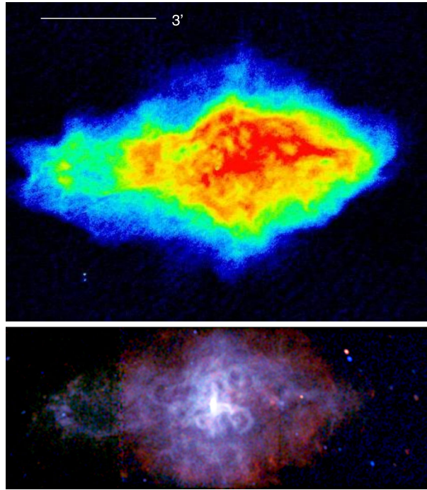
Fig. 7 Top : VLA image of 3C 58 at 1.4 GHz (Reynolds and Aller 1988). Bottom : Chandra X-rays (Slane et al. 2008). Note the close correspondence between detailed features, and the similar maximum extent in radio and X-rays
