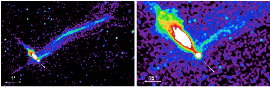
Fig. 36 Chandra ACIS image of the Lighthouse PWN (0.5–8 keV, 300 ks) created by PSR J1101-6101 ( \dot{E} = 1.4 \times 10^{36} erg s ^{-1} , \tau_{\text{sd}} = 116 kyr) moving from the SNR MSH 11-61A (Pavan et al. 2016). The image shows a bright tail behind the fast-moving pulsar ( V_{\perp} \sim 1000d_7 km s ^{-1} ) and an 11 d_7 pc long jet-like feature, possibly another example of a “misaligned outflow”
