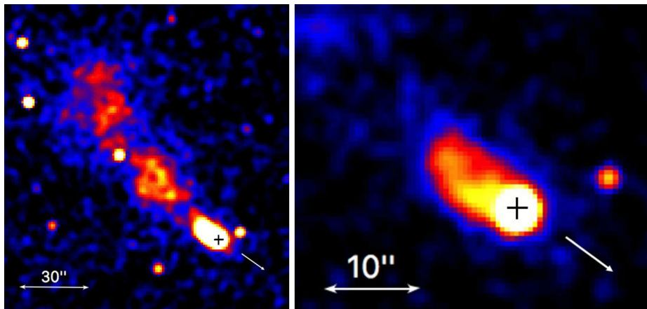
Fig. 33 Summed 0.3–6 keV Chandra ACIS images of the entire J1741-2054 PWN ( left ) and the leading bright component ( right ) from 5 observations in 2013 (282 ks total exposure). Black crosses show the pulsar position, white arrows show the direction of proper motion
