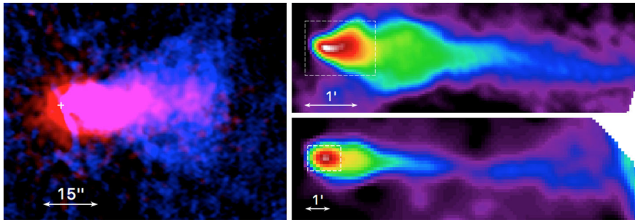
Fig. 24 Left: Composite X-ray ( red ; ACIS) and radio ( blue ; VLA, 1''07 beam) image of the Mouse PWN. The pulsar position is shown by the white cross . Right: VLA radio images ( top : 11'' beam, bottom : 32'' beam) showing the extended tail of the Mouse. The field of view of the left image is shown by the dashed white box in the lower right panel. The radio images were obtained from the NRAO VLA Archive
