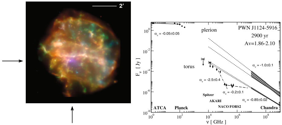
Fig. 20 Left: The shell SNR G292.0+1.8, with the pulsar indicated and the PWN in blue (Park et al. 2007). Right: SEDs of the entire PWN and of the torus [seen in VLT images at H and K_s bands; Zharikov et al. (2013)]. The torus spectrum is complex, but the PWN could be described by a double power-law with a single spectral break around 100 GHz. However, the steepening \Delta is almost 1
