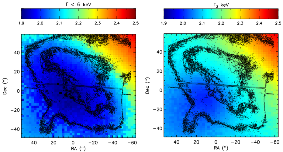
Fig. 12 Left: Crab photon index \Gamma below 6 keV; right: \Gamma above 10 keV (Madsen et al. 2015). Contours are from Chandra (Mori et al. 2004)
