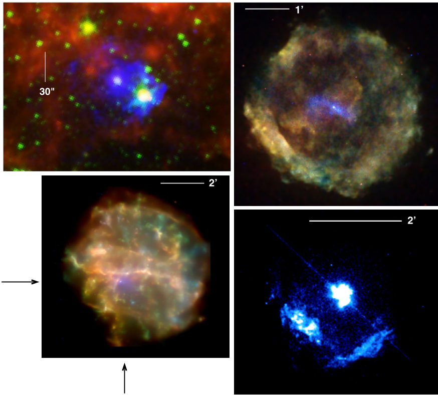
Fig. 2 Upper left: B0540-693 in the Large Magellanic Cloud (Williams et al. 2008). Red, Spitzer 8 \mu\text{m} ; green, Spitzer 3.6 \mu\text{m} ; blue, Chandra 0.5–8 keV. The pulsar and surrounding PWN is barely resolved at the center of the frame, just above and to the left of the bright foreground star. Upper right: G11.2-0.3 with Chandra (Borkowski et al. 2016). Red: 0.6–1.2 keV; green, 1.2–3.3 keV; blue, 3.3–8 keV. The PWN is visible in blue. Lower left: G292.0+1.8 with Chandra (Park et al. 2007). Red: 0.3–0.8 keV; green, 0.8–1.7 keV; blue, 1.7–8 keV. The PWN is the purplish region slightly SE of the center, and the pulsar (indicated by arrows) is at its NE edge. Lower right: Kes 75 with Chandra (Gavriil et al. 2008). The pulsar is highly piled up, as the readout streak indicates
