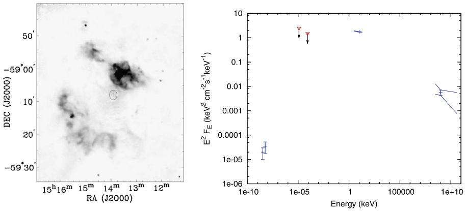
Fig. 17 Left: Radio image of MSH 15-52 at 1.3 GHz with ATCA (Gaensler et al. 1999). The bright horseshoe to the N is RCW 89. There is little evidence of the PWN; the cross marks the pulsar location. Right: SED for MSH 15-52. Radio: Gaensler et al. (2002). IR upper limits are from Koo et al. (2011). X-rays: An et al. (2014). TeV: Aharonian et al. (2005)
