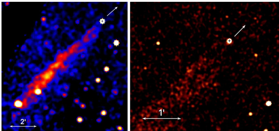
Fig. 35 Left : Merged Chandra ACIS image of the tail behind PSR J0357+3205 (0.5–6 keV, 4 observations, 136 ks total exposure). Right : Zoomed-in part of the same image showing the lack of tail emission in the pulsar vicinity
