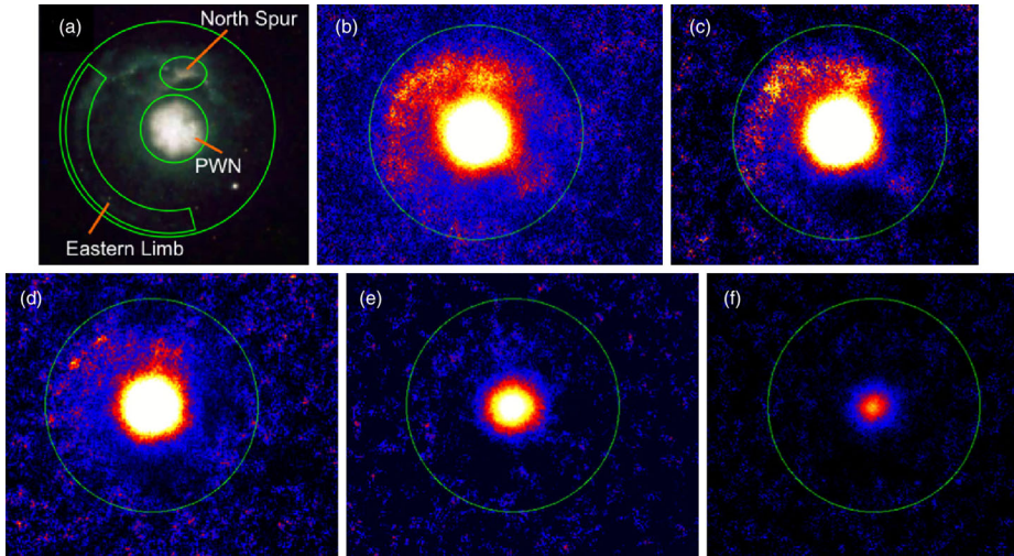
Fig. 14 (a): Chandra image of G21.5-0.9 between 3 and 6 keV (Matheson and Safi-Harb 2005). (b)–(f): Deconvolved NuSTAR images in various bands: (b) 3–6 keV; (c) 6–10 keV; (d) 10–15 keV; (e) 15–20 keV; and (f) 20–25 keV. The green circles in panels (b) through (f) have radii of 165''
