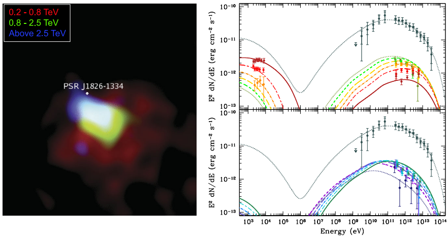
Fig. 40 Left: Three-color 3^\circ -large image of HESS J1825-137 as observed with H.E.S.S. in different energy bands (Funk et al. 2008) showing the shrinking of the nebula with increasing energy. Right: Broadband spectra from the whole PWN (slate data points and dotted line) and from different wedges in HESS J1825-137 with a color scale evolving from dark red (inner region) to green, blue and violet (outer region), as defined in Aharonian et al. (2006a). Lines represent the best-fit model presented in Van Etten and Romani (2011) (see text for more details)
