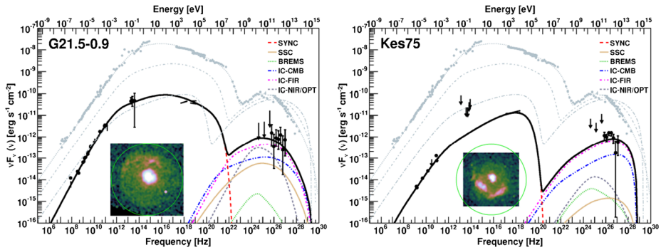
Fig. 39 Broadband spectra of G21.5-0.9 (left) and Kes 75 (right) with the best-fit models from Torres et al. (2014) shown as solid lines . The grey dots and lines correspond to the multi-wavelength data and the associated models (at different ages) for the Crab nebula. Chandra X-ray images of these two PWNe with the typical H.E.S.S. PSF depicted as a green circle are also shown
