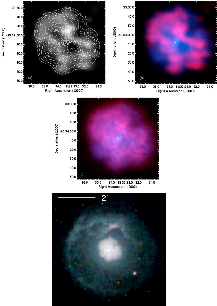
Fig. 13 G21.5-0.9 in radio and X-rays (Matheson and Safi-Harb 2010). Upper left: radio (greyscale; 22.3 GHz from the Nobeyama Millimeter-Wave Array, resolution 8'' (Fuerst et al. 1988) and X-rays ( Chandra contours; Matheson and Safi-Harb 2010). Upper right: 22.3 GHz data in red, Chandra in blue. Center: 4.75 GHz radio (VLA; Bietenholz and Bartel 2008) in red, same X-rays in blue. Bottom: Chandra (Matheson and Safi-Harb 2010)
