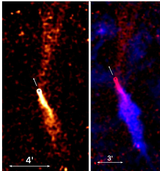
Fig. 30 Left: Chandra ACIS image of the J1509-5850 PWN (0.5–8 keV, 374 ks) showing the southwest tail and the misaligned outflow toward the north. Right: Combined Chandra ACIS (red) and VLA (blue) image of the same PWN. The arrows show an assumed direction of proper motion
