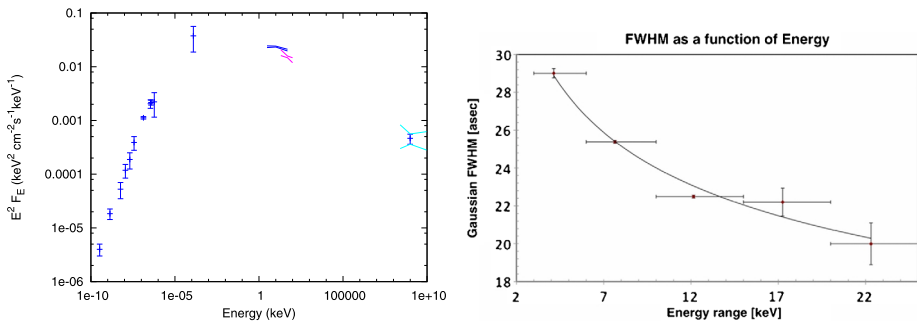
Fig. 15 Left : G21.5-0.9 SED (PWN only). Radio–mm points from Salter et al. (1989); IR point from Zajczyk et al. (2012); blue bowtie, NuSTAR (Nynka et al. 2014); magenta bowtie, INTEGRAL (de Rosa et al. 2009); TeV bowtie in cyan, H.E.S.S. (Djannati-Ataï et al. 2008). Right : Shrinkage of G21.5-0.9 with photon energy (Nynka et al. 2014)
