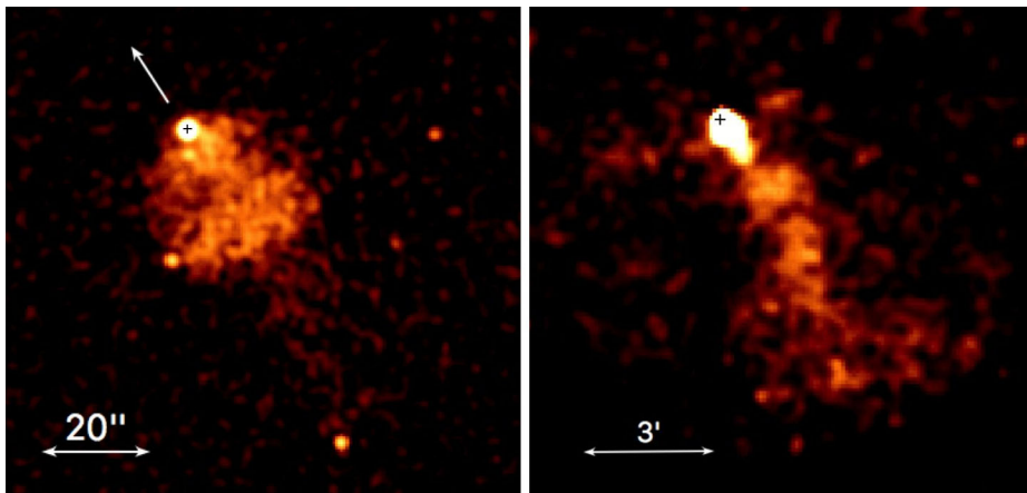
Fig. 32 Chandra ACIS images of the B0355+54 PWN (0.5–8 keV, 395 ks). Left : The compact PWN in the pulsar vicinity (the Mushroom). Right : The large-scale PWN, including the diffuse tail and the “whiskers”. The arrows show the direction of the proper motion
