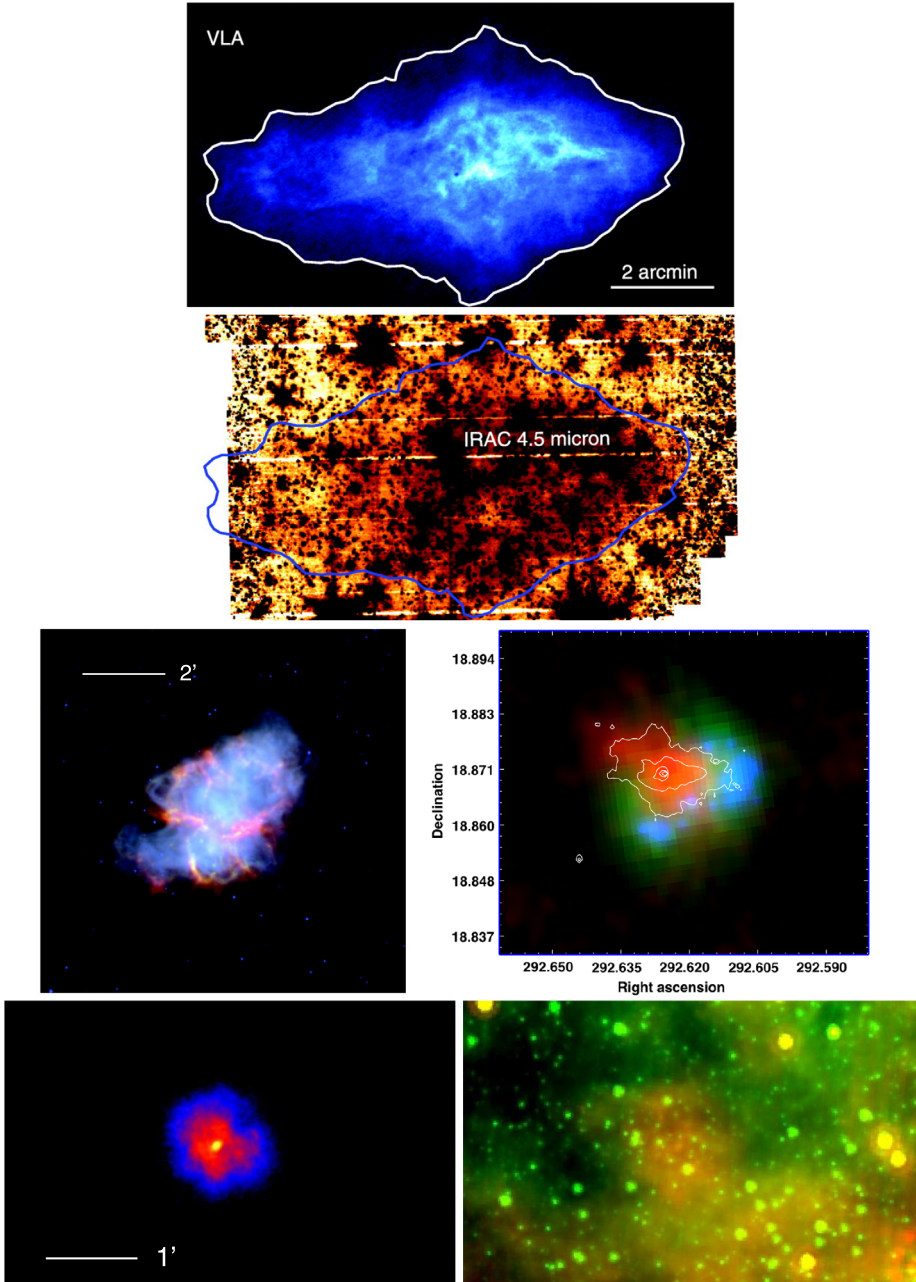
Fig. 5 Top: 3C 58 (Slane et al. 2008). ( Upper: radio, VLA at 1.4 GHz, Reynolds and Aller 1988; lower: IR, Spitzer at 4.5 \mu\text{m} .) Middle left: Crab Nebula (Temim et al. 2006). Red , 24 \mu\text{m} (mainly [O IV] at 26 \mu\text{m} ); green , 8 \mu\text{m} (mainly [Ar II] at 7 \mu\text{m} ); blue , 3.6 \mu\text{m} (mainly synchrotron continuum). Middle right: G54.1+0.3 (Temim et al. 2010). Contours , X-ray. Red , radio. Green , 70 \mu\text{m} . Blue , 24 \mu\text{m} . Lower: G21.5-0.9 (Zajczyk et al. 2012). Left: Chandra image. Right: Red , 24 \mu\text{m} ; green , 8 \mu\text{m}
