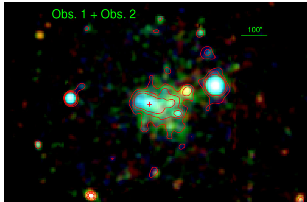
Fig. 44 X-ray image of the region of Swift J1834.9-0846 obtained with the XMM-Newton satellite (from Younes et al. 2016). The cross indicates the position of the magnetar. The colors code the X-ray energy ( red 2–3 keV, green 3–4.5 keV, 4.5–10 keV blue ). The contours are at the 2.5, 3.0, and 3.5 \sigma level. For a distance of 4 kpc, 100'' correspond to \sim 2 pc ( horizontal bar )
