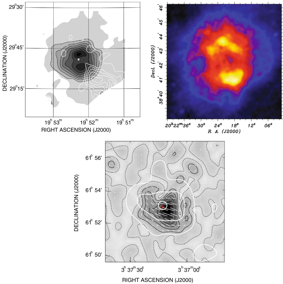
Fig. 4 Three PWNe with steep radio spectra. Upper left : DA 495 (G65.7+1.2) at 1.4 GHz. White contours : a background H II region. Asterisk : a compact X-ray source (Kothés et al. 2008). Upper right : G76.9+1.0 (Arzoumanian et al. 2011) at 1.4 GHz. Almost invisible contours of extent about 40'' near the center show the X-ray nebula. Bottom : G141.2+5.0 at 1.4 GHz in polarized intensity ( greyscale ) with contours indicating total intensity (Kothés et al. 2014), and the red cross indicating a pointlike X-ray source (Reynolds and Borkowski 2016)
