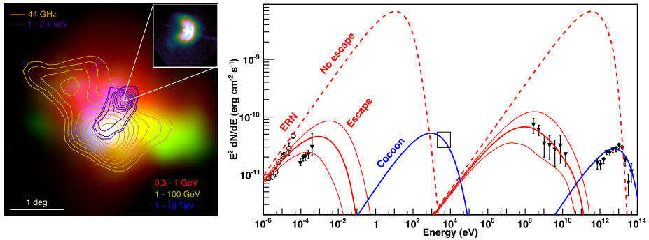
Fig. 41 Left: multi-wavelength picture of Vela PWN. The 4°-wide three-color image (in Galactic coordinates) is composed of the 0.3–1 GeV (red) and 1–100 GeV (green) emission measured with Fermi -LAT (Grondin et al. 2013), and of the 1–10 TeV (blue) emission detected with H.E.S.S. (Abramowski et al. 2012). Contours represent the 44 GHz radio emission measured by Planck (Planck Collaboration et al. 2016) and the X-ray emission above 1 keV observed with ROSAT (in blue). The well-known X-ray compact nebula around the Vela PSR is shown in the inset on the upper right corner ( Chandra /ACIS 0.3–10 keV image). Right: broadband spectrum of Vela PWN (ERN: Extended Radio Nebula) with (solid lines) and without (dashed lines) the assumption of particle escape throughout its evolution, according to Hinton et al. (2011)
