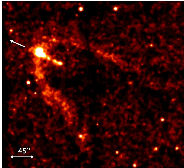
Fig. 26 Combined Chandra ACIS image of the Geminga PWN (0.5–8 keV, 540 ks). The arrow shows the direction of the pulsar’s proper motion
