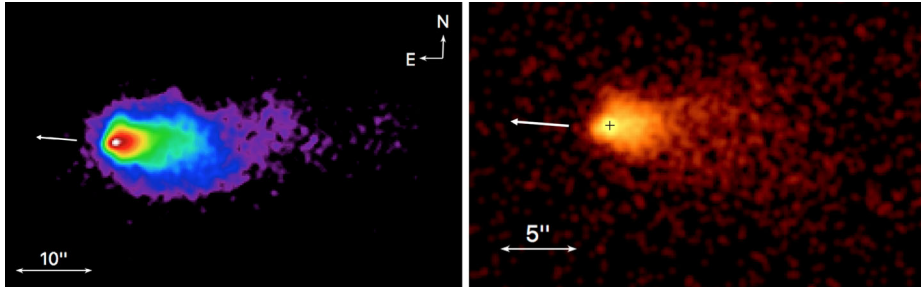
Fig. 23 Left: Merged image from 5 Chandra ACIS observations of the Mouse (0.5–8 keV, 154 ks exposure). Right: Chandra HRC image of the Mouse (58 ks exposure). The cross in the right image marks the pulsar position; the arrows show the direction of proper motion
