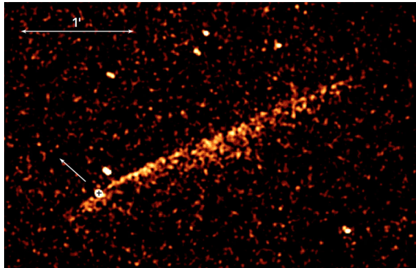
Fig. 28 Combined Chandra ACIS image (0.5–8 keV, 195 ks total exposure) of PSR B2224+65 and its misaligned outflow, in a coordinate frame moving with the pulsar. The image is a combination of two images separated by an interval of 6 years, during which the pulsar moved 1'' on the sky
