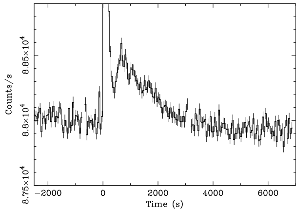
Fig. 42 High-energy ( >80 keV) light curve of the 27 December 2004 giant flare of SGR 1806-20 measured with the INTEGRAL satellite (from Mereghetti et al. 2005). After the bright flare truncated in the plot (reaching >2 \times 10^6 counts s^{-1} ) a long tail of hard X-ray emission, which peaks at t \sim 500 s and lasts more than one hour is clearly visible
