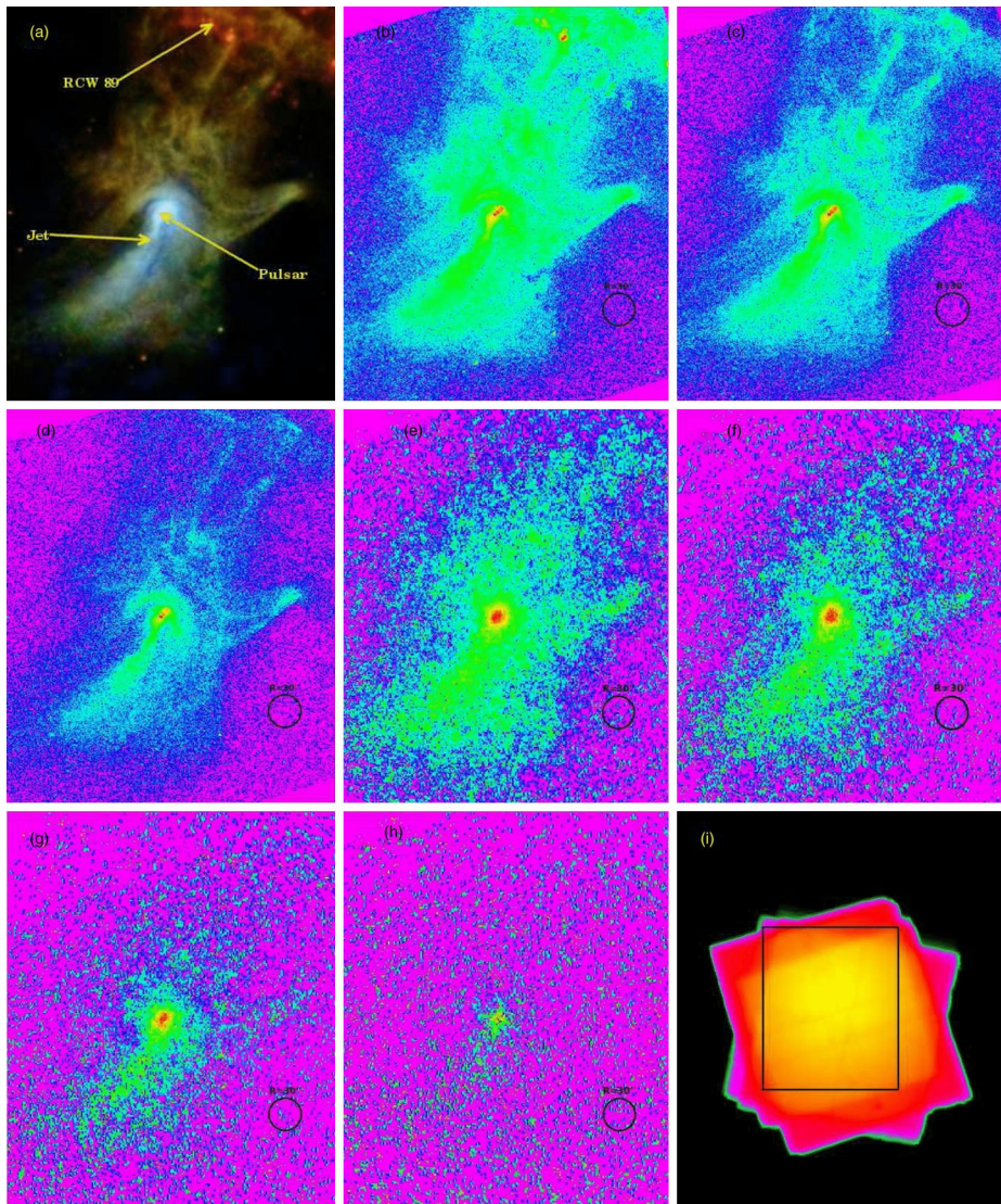
Fig. 16 MSH 15-52 with Chandra and NuSTAR (An et al. 2014). From left to right, top to bottom: Chandra + NuSTAR , 0.5–40 keV; Chandra , 0.5–2 keV; Chandra , 2–4 keV; Chandra , 4–7 keV; NuSTAR , 3–7 keV; NuSTAR , 7–12 keV; NuSTAR , 12–25 keV; NuSTAR , 25–40 keV; NuSTAR exposure map. All frames except the last are 10' \times 12'
